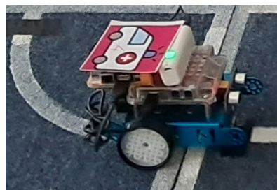
Figure 7: Mbot with Raspberry Pi 3 and battery on its top
