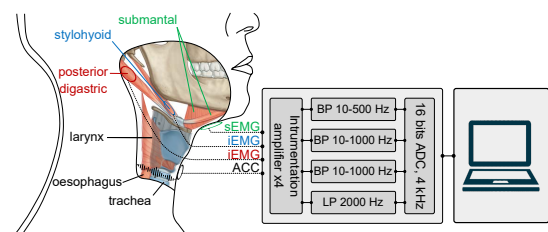
Fig. 1. Sensors locations, anatomical structures and acquisition set up. EMG: electromyography, sEMG: surface EMG, iEMG: intramuscular EMG, ACC: accelerometer, BP: band-pass, LP: low-pass. ADC: analogue digital converter.
