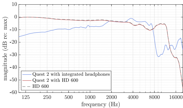
Figure 6: Frequency response (1 channel) of the Quest 2 integrated headphones, measured with a KU100 dummy-head. The logarithmic sine-sweep used as a stimulus was uploaded to the Quest Unity using the PCM (lossless) decompression algorithm. For comparison, the response of the Quest 2 connected (3.5 mm jack output) to a HD 600 headset has been added (“Quest 2 with HD 600”), as well as that of the HD 600 alone, using the same unity application, not running on the Quest 2 but on a computer.
