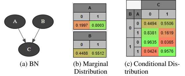
Figure 1: (a) Example of a BN composed of three variables A , B and C . (b) Marginal distributions associated to A and B . (c) CPT associated to C : in this example the probabilities of C 's values (columns) depend on A and B 's values (rows).
