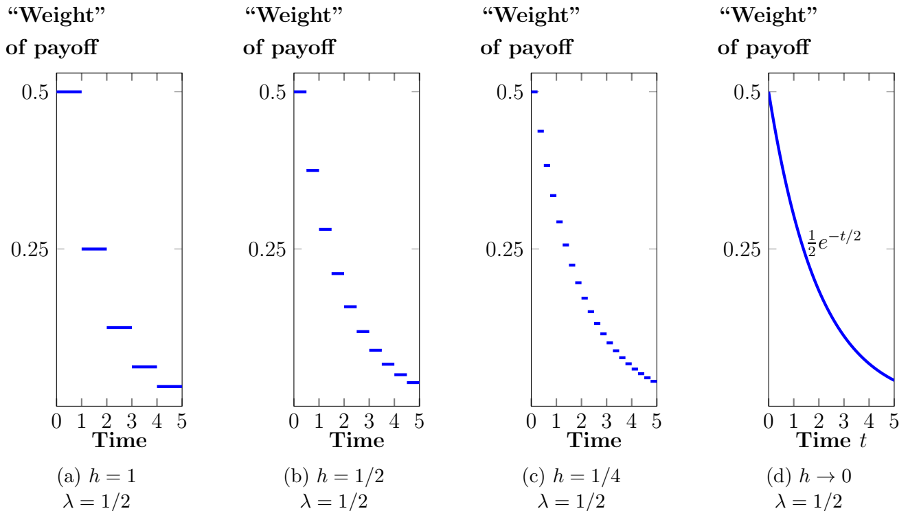
Figure 4: A demonstration of how the weight of each stage in a stochastic game in which each stage has duration h tends to the weight function \frac{1}{2}e^{-t/2} of a continuous-time game. (In (a),(b),(c), the weight \lambda(1 - \lambda h)^{n-1} of n -th stage is shown during the time t \in [(n - 1)h, nh] ).
