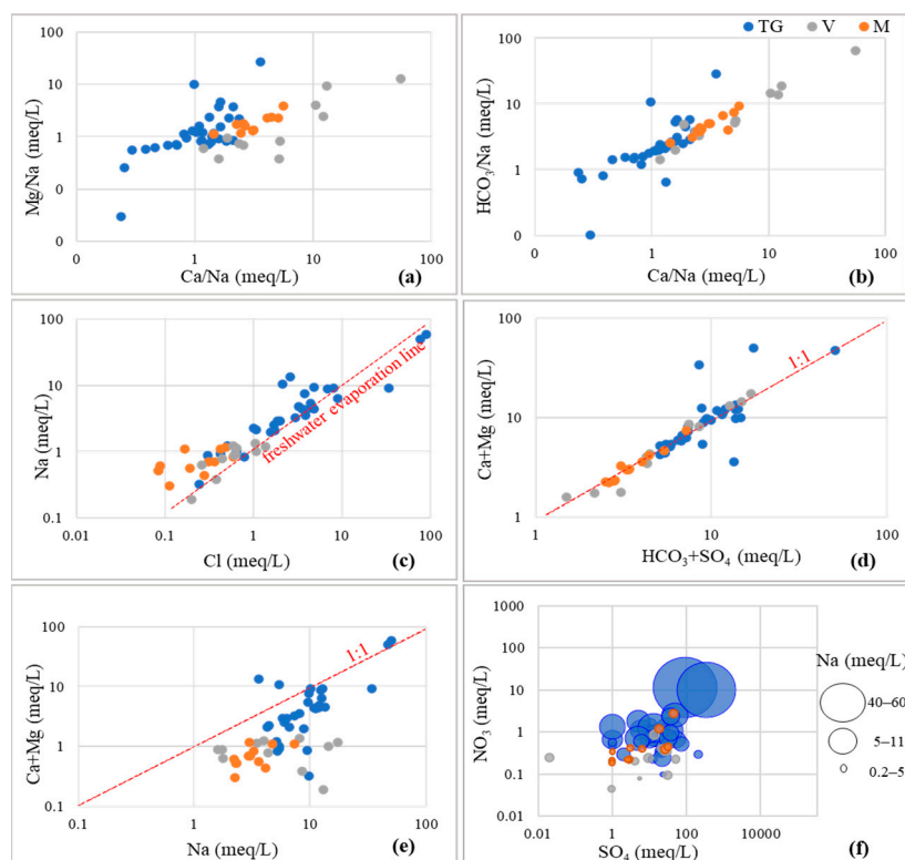
Figure 7. Ionic ratio plots relative to groundwater samples from M = Mouriki basin, TG = Eastern Thermaikos Gulf, and V = Upper Volturno basin: (a) (Mg/Na)/(Ca/Na) , (b) (HCO_3/Na)/(Ca/Na) , (c) Na/Cl , (d) (Ca + Mg)/(HCO_3 + SO_4) , (e) (Ca + Mg)/Na , and (f) NO_3/SO_4 with Na.
