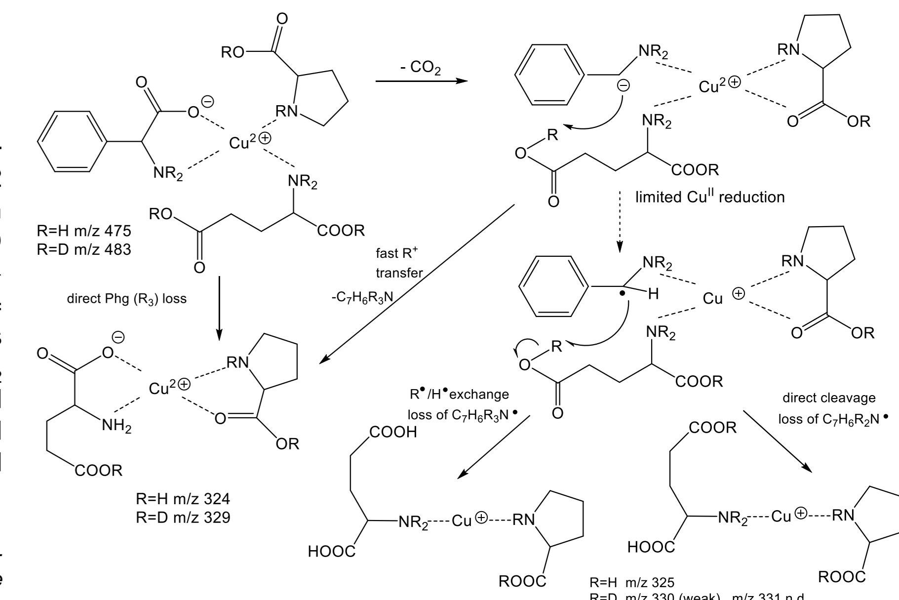
Scheme 1. Proposed competitive direct Pgly and stepwise [Pgly-H]^{\bullet} losses: unexpected H/D • radical exchanges and origin of the enantioselective reduction decrease.
