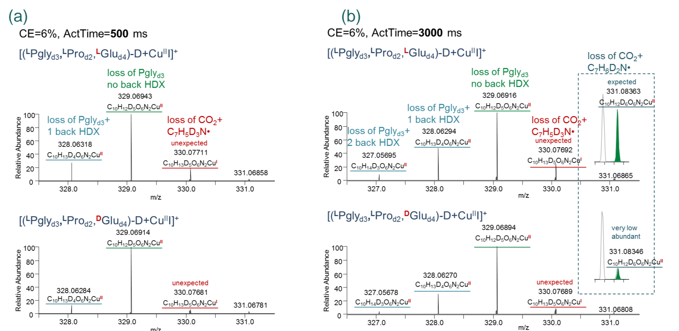
Figure 6. Comparison of the regions of interest of the product ion spectra of homochiral [(L)Pgly_{d3}+LPro_{d2}+L(Glu_{d4})-D+Cu^{II}]^+ and heterochiral [(L)Pgly_{d3}+LPro_{d2}+D(Glu_{d4})-D+Cu^{II}]^+ CQC ions (m/z 493) activated during (a) 500 ms and (b) 3000 ms in CID mode at NCE = 6%.
