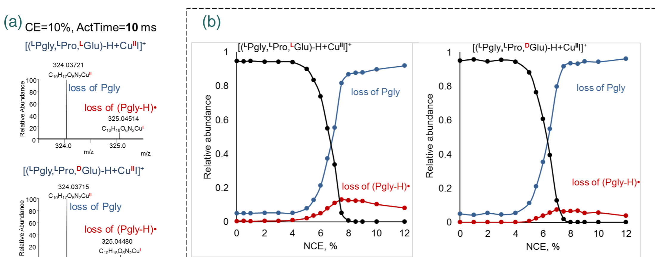
Figure 4. (a) Region of interest of product ion spectra (CID mode, NCE = 10%, ActTime = 10 ms) of homochiral [(L)Pgly+LPro+LAA-H+Cu^{II}]^+ and heterochiral [(L)Pgly+LPro+DAA-H+Cu^{II}]^+ CQC ions (m/z 475) and (b) energy resolved CID breakdown curves for diastereomeric CQC ions with the relative abundances of survivor precursor ions and competitive product ions normalized to the total ionic current.
