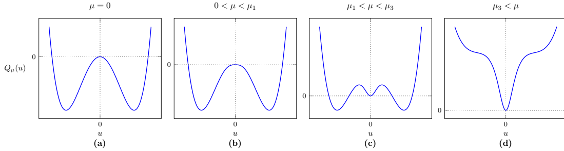
Figure 2: Effect of the perturbation parameter \mu on the potential Q_\mu(u) defined by (11). (a)-(b) For 0 \leq \mu < \mu_1 , Q_\mu(u) admits two local minima. (c) For \mu_1 < \mu < \mu_3 , it admits three local minima. (d) For \mu_3 < \mu , it admits a unique global minimum.
