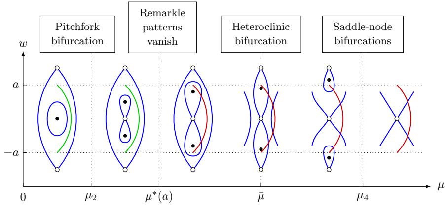
Figure 13: Bifurcation diagram showing the dynamics of the Hamiltonian system (33) obtained with a monotone and piecewise continuous inverse \psi_\mu of q_\mu . A pitchfork bifurcation occurs at \mu_2 ; particular discontinuous patterns connecting -a to a exist for \mu < \mu^*(a) but vanish for \mu > \mu^*(a) (hence they are depicted in green for \mu < \mu^*(a) and in red for \mu > \mu^*(a) ); a bifurcation of heteroclinic orbits occurs at \bar{\mu} ; finally, two simultaneous saddle-node bifurcations take place at \mu_4 .
