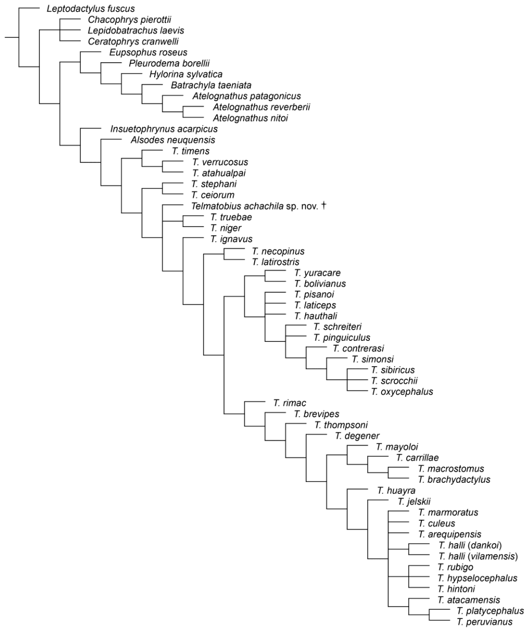
FIG. S9. Topology of the strict consensus of eight MPTs (322.430 steps; CI = 0.368; RI = 0.725) obtained with dataset B17 under implied weights with k = 8-9 and multistate characters unordered.
