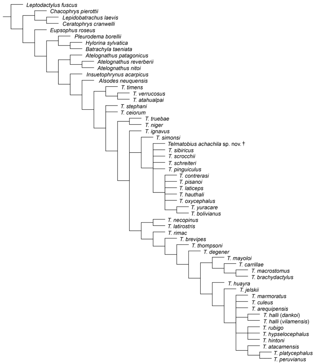
FIG. S8. Topology of the strict consensus of 100 MPTs (328.332 steps; CI = 0.361; RI = 0.720) obtained with dataset B17 under implied weights with k = 8-9 and multistate characters ordered.
