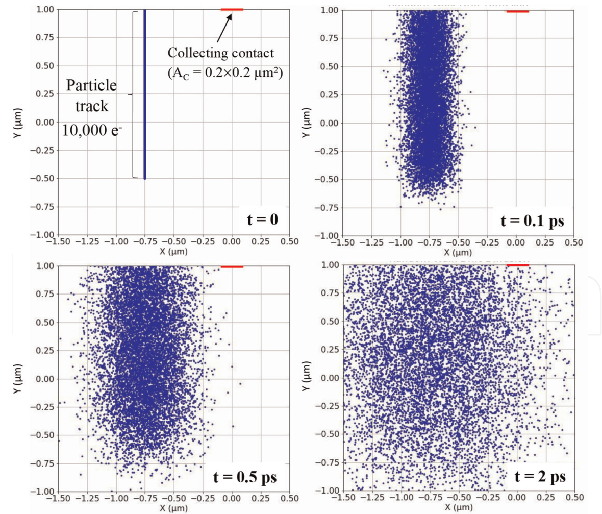
Figure 6. Distributions of charges in a vertical section along the x-y plane ( z = 0 ) at t = 0, 0.1, 0.5 , and 2 ps after the deposition of 10,000 electrons along a 1.5\text{-}\mu\text{m} length track located at 0.75\text{ }\mu\text{m} from the contact. Other simulation parameters are the same as reported in the caption of Figure 3.
