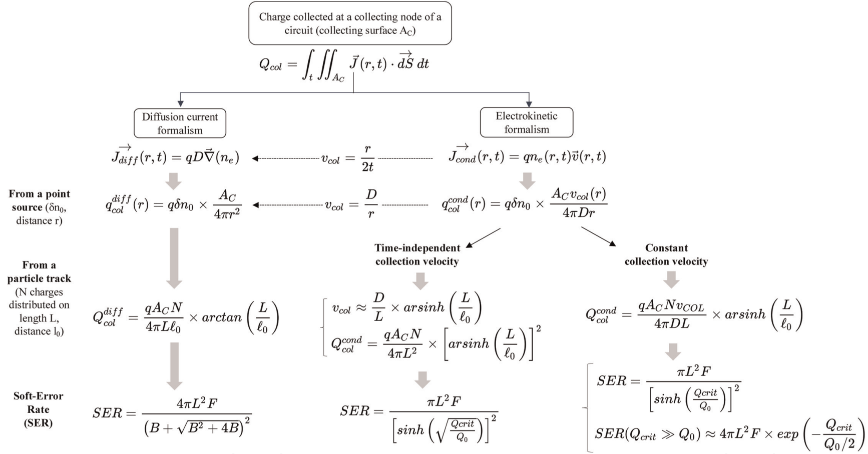
Figure 11. Summary of the diffusion-collection model developed in this work.
