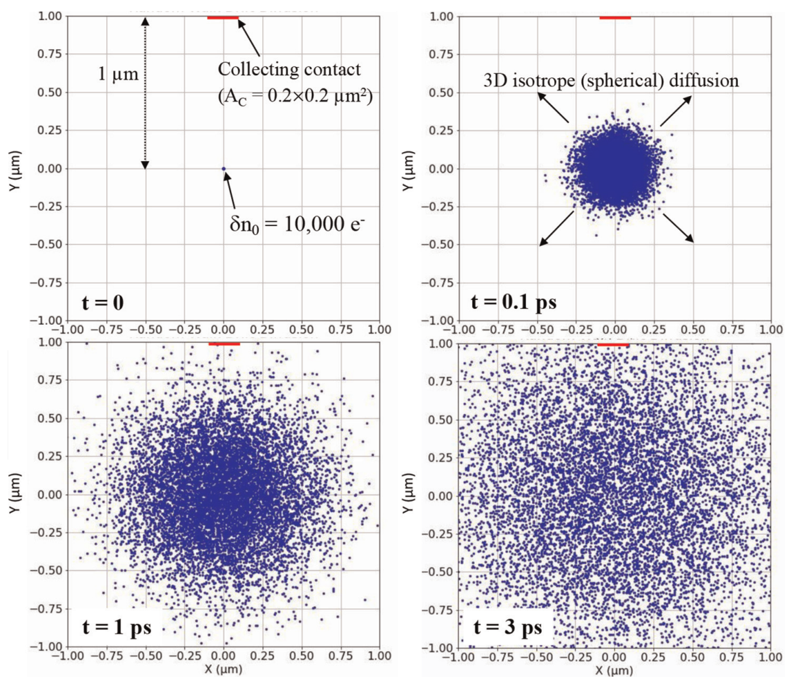
Figure 3. Distributions of charges in a vertical section along the x - y plane ( z = 0 ) at t = 0, 0.1, 1 and 3 \text{ ps} after the deposition of 10,000 electrons at position (0, 0, 0) . Charges are transported following Eq. (10) with D^* = 533 \text{ cm}^2/\text{s} , \Delta t = 0.1 \text{ ps} , and E_0 = 0 (pure diffusion law). The surface of the collecting contact is in the x - z plane, perpendicular to the figure.
