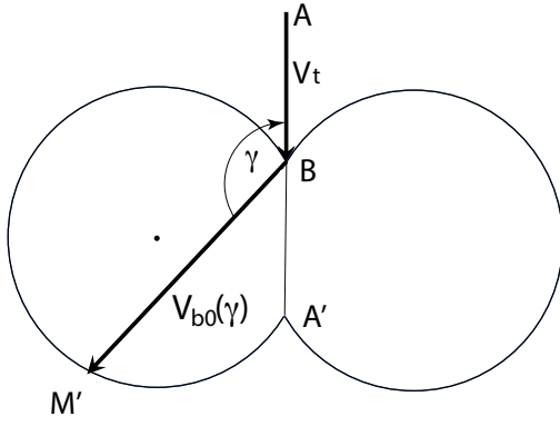
Figure 5: Polar diagram V_{b0}(\gamma) under both tacks for a boat sailing at constant apparent wind angle \beta_0 = 30^\circ . Points A' and M' are symmetrical of A and M (see figure 4) with respect to point B .
