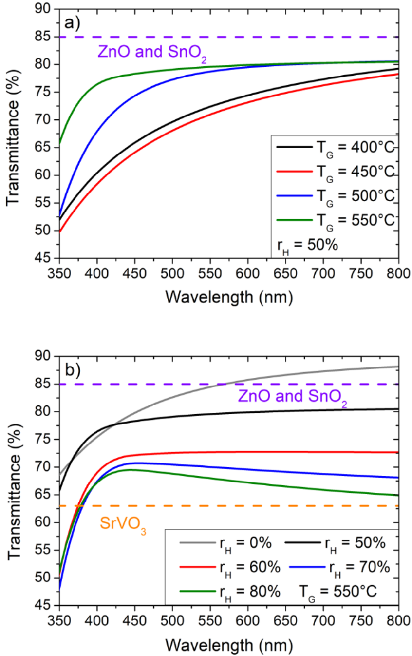
Figure 13: Evolution of transmittance as a function of the wavelength for, a) different values of T_G with r_H = 50\% , b) different values of r_H with T_G = 550^\circ\text{C} .
