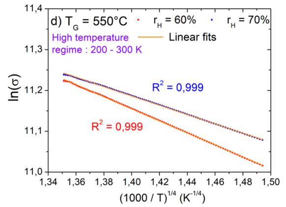
Figure 9: a) carrier mobility as a function of temperature for different values of r_H and T_G = 550^\circ\text{C} , b) carrier concentration as a function of temperature for different values of r_H and T_G = 550^\circ\text{C} , c) Plot of \ln(\sigma) as the function of 1000/T for T between 200 and 300 K and for different values of r_H and T_G = 550^\circ\text{C} , d) Plot of \ln(\sigma) as the function of (1000/T)^{1/4} for T between 200 and 300 K and for different values of r_H and T_G = 550^\circ\text{C} .
