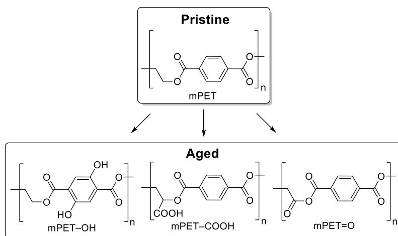
Figure 12. Molecular structure of pristine and aged model PET monomers.
