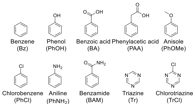
Figure 2. Organic pollutant molecular models.
