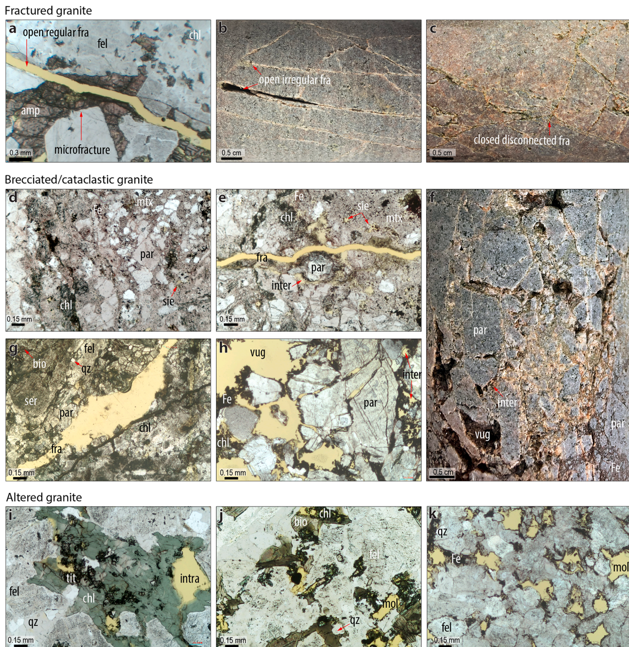
Fig. 4. Drilling core photographs (b, c, and f) and thin-section images in plain polarized light (a, d, e, g, h, i, j, k) showing the minerals, textures, structures, and pore types of the granitic reservoirs identified in this study. Abbreviations are: tit (titanite), fel (feldspar), qz (quartz), amp (amphibole), bio (biotite), chl (chlorite), epi (epidote), ser (sericite), Fe (iron oxides, including magnetite, hematite, and ilmenite), py (pyrite), par (particles, referring to cataclastic grains >1mm in size), mtz (matrix, referring to cataclastic grains <1mm), fra (fracture pore), inter (interparticle pore), intra (intracrystal pore), sie (sieve pore), vug (vug pore), and mol (moldic pore). Rock porosity is highlighted in yellow.
