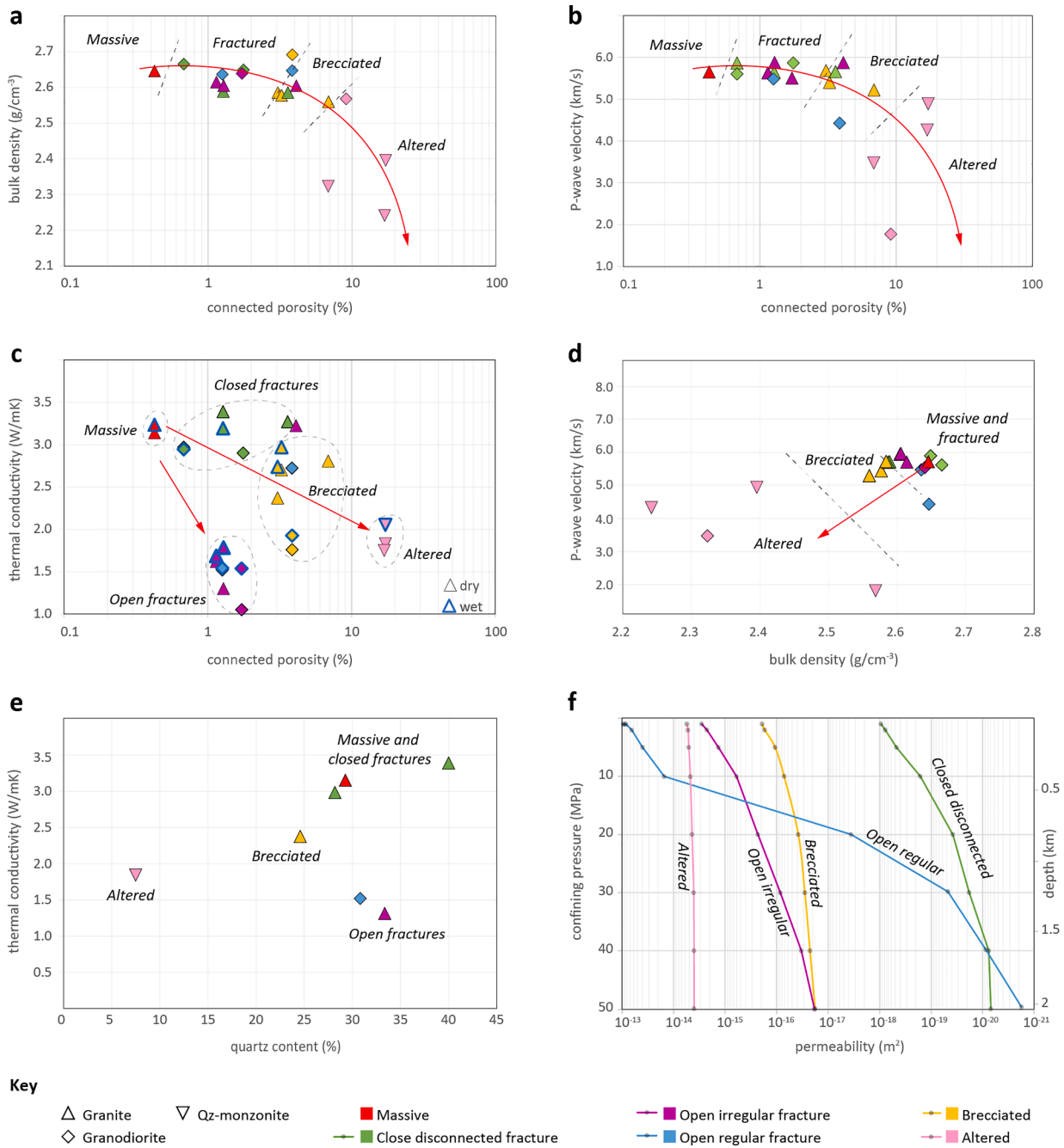
Fig. 6. Petrophysical and thermal data of the granitic rocks investigated in our study. The observed heterogeneity of these rocks is mainly controlled by their distinctive pore network, which in turn, is determined by brittle deformation (fracturing and brecciations) and mineral alteration processes. Depths estimation in (f) considers a crystalline setting in which the lithostatic load is 2.6kg/cm 3 .
