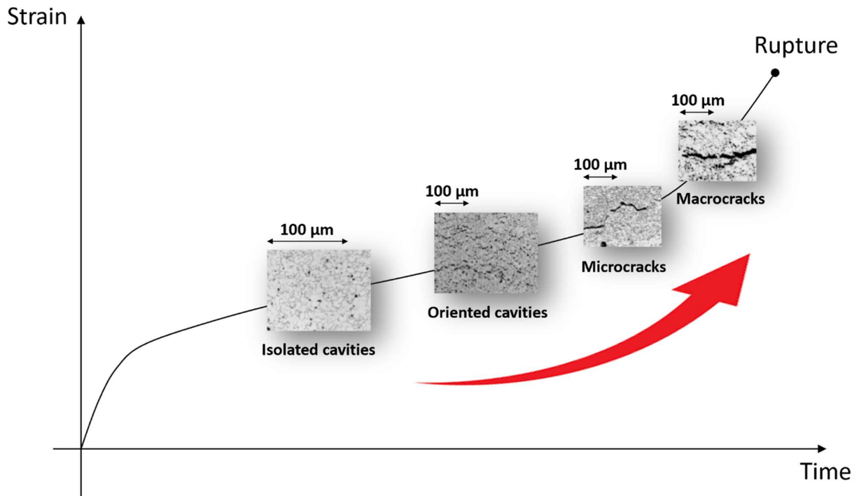
Fig. 2 – Strain vs. time, illustration of the creep effect
