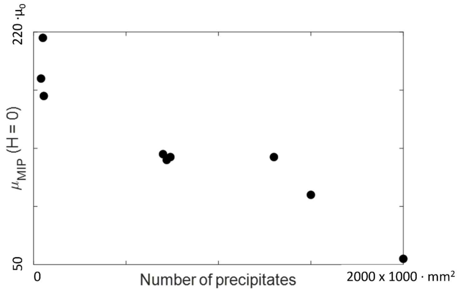
Fig. 7 – Typical evolution of the magnetic incremental permeability at H = 0 as a function of the number of precipitates.
