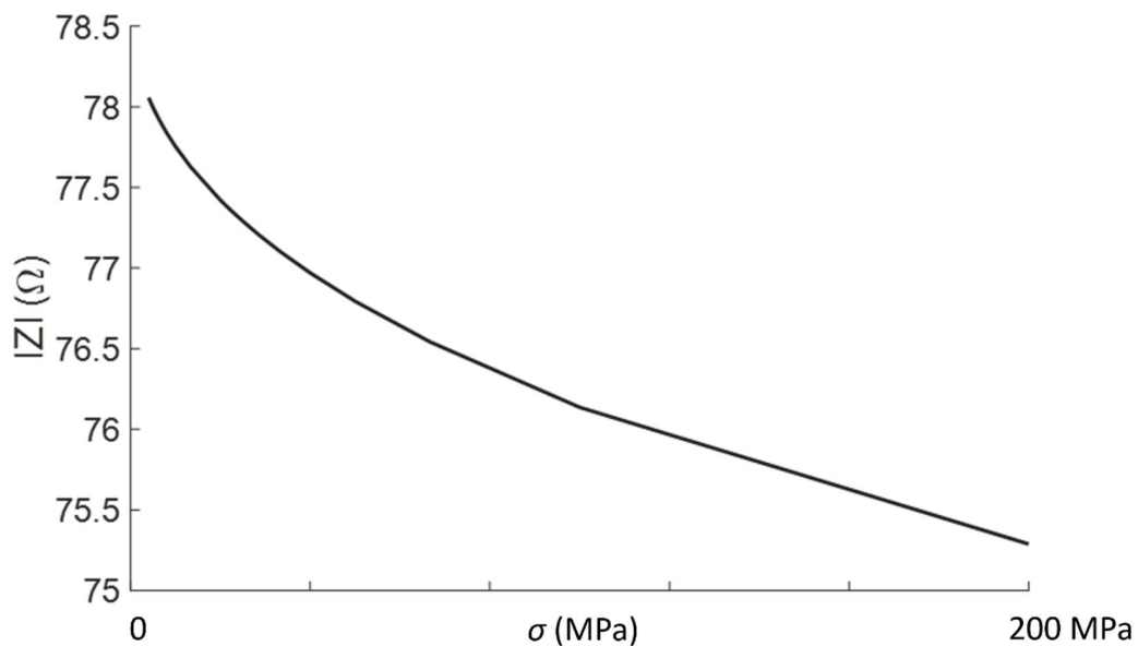
Fig. 6 – Illustration of a uniaxial homogeneous stress influence on the impedance modulus of an eddy current sensor.
