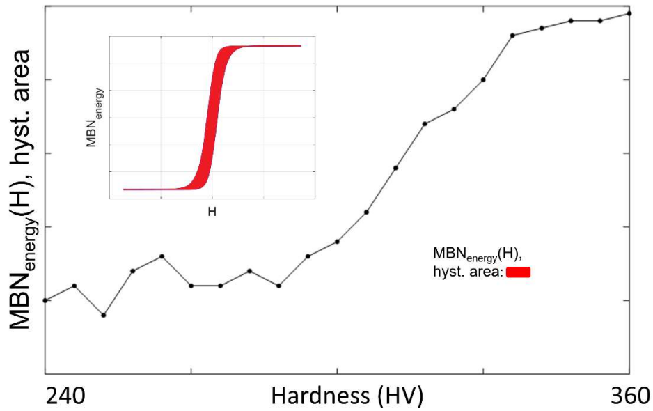
Fig. 8 – Typical evolution of the MBN_{energy}(H) hysteresis loop area as a function of hardness.
