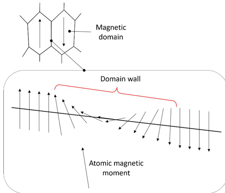
Fig. 3 – Orientation change of atomic magnetic moment in a Bloch type domain wall
