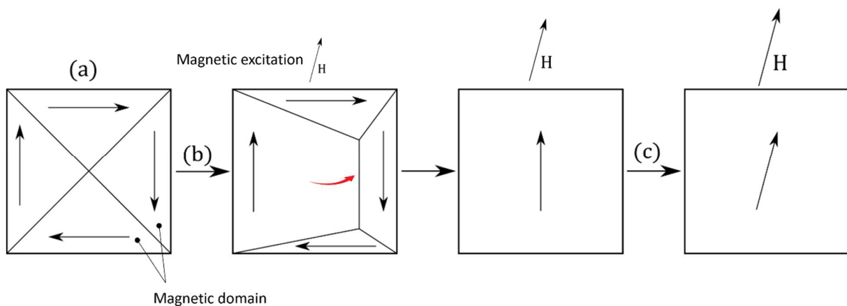
Fig. 4 – Schematic illustration of the magnetization process. (a) Demagnetised state (b) Domain wall motion (c) Magnetisation rotation. In practice, the two mechanisms can occur simultaneously.
