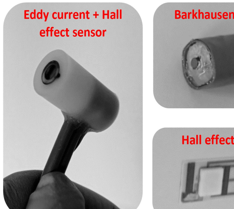
Fig. 5 – Illustration of sensors, specimens, and experimental setups used to observe the magnetization mechanisms at a laboratory scale.
