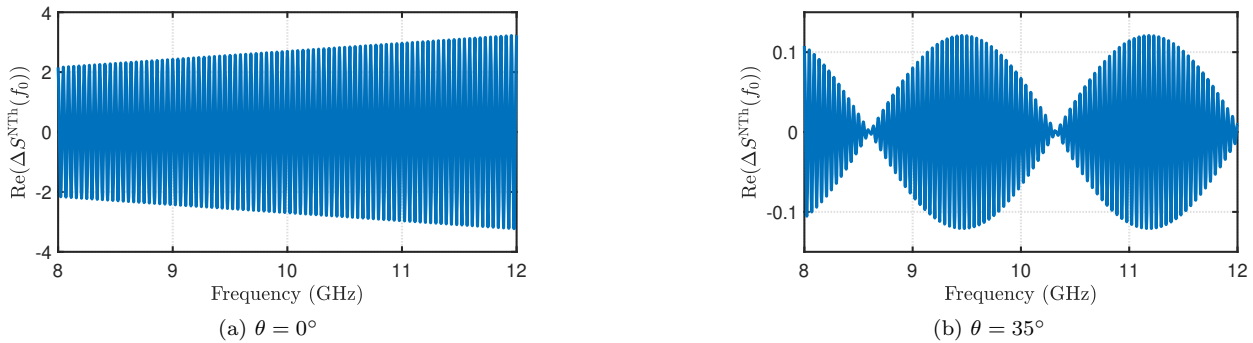
Figure 2: Real part of the theoretical noiseless difference of S-parameters ( \Delta S^{\text{NTh}}(f_0) ) in absence and presence of a metallic rectangular plate at (a) \theta = 0^\circ and (b) \theta = 35^\circ .
