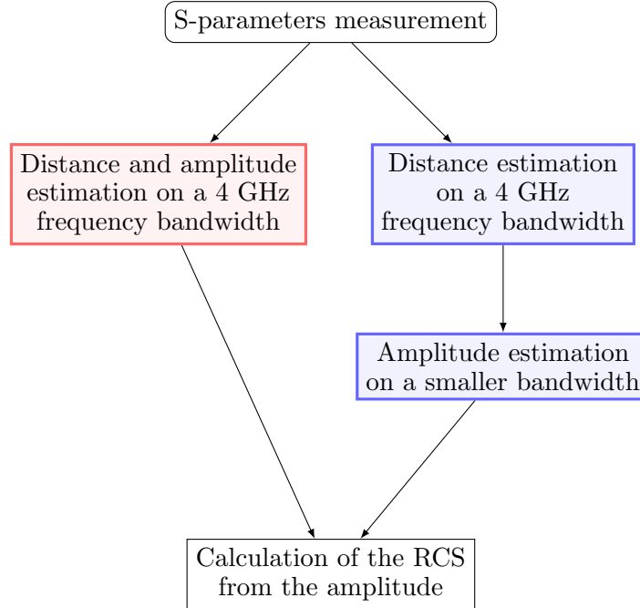
Figure 12: Flow-chart of the one-step method (left) and of the two-step method (right) in an RC.
