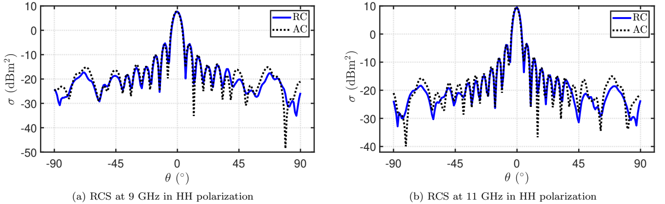
Figure 16: Comparison of RCS extracted from RC measurements using a distance bandwidth of 4 GHz between 8 GHz and 12 GHz and an amplitude bandwidth of 0.9 GHz for different central frequencies (9 GHz and 11 GHz) and RCS obtained from AC measurements according to the plate position in the -90^\circ to +90^\circ azimuth range and in the HH polarization.
