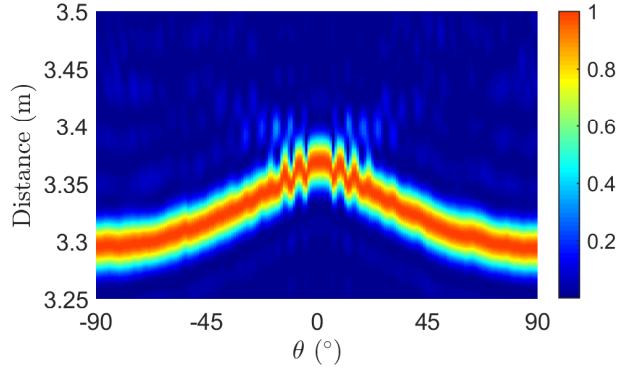
Figure 8: Amplitude of the sinusoidal regression fit in the 3.25 – 3.50 m range as a function of the azimuth angle ( -90^\circ \leq \theta \leq +90^\circ ) in the VV polarization considering the largest frequency bandwidth (4 GHz). The amplitude is normalized to its maximal value at each angle.
