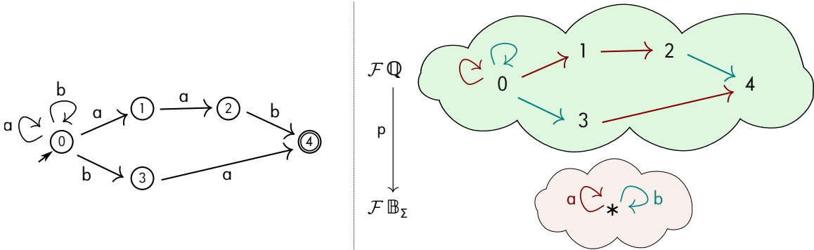
Figure 4: Left: an N DFA represented with a traditional state-diagram. Right: the bare N DFA as a finitary ULF functor p : \mathcal{F} \mathcal{Q} \rightarrow \mathcal{F} \mathbb{B}_\Sigma . (We do not label the generators of \mathcal{F} \mathcal{Q} or indicate composite arrows, and we use colors to indicate the images of the generators in \mathcal{F} \mathbb{B}_\Sigma .)
