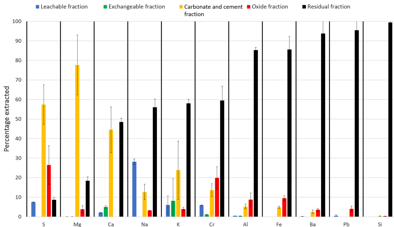
Fig. 5. Distribution of major and some minor and trace elements in the fractions of the sequential extraction experiment conducted on T-RX. Elements are ordered following the trend of increasing residual fraction.
