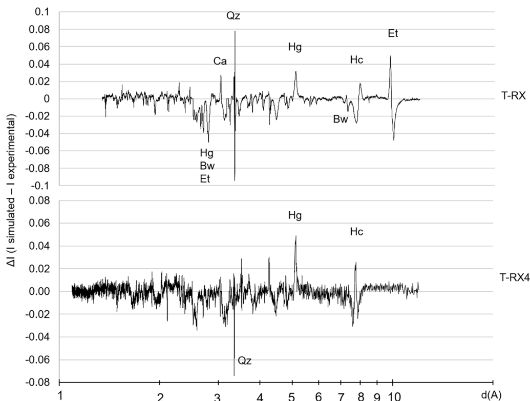
Fig. 3. Residual signals of Rietveld analysis on T-RX and T-RX4 materials. \Delta I is the intensity difference between simulated and experimental XRD traces. \Delta I is normalised to 1. Et: ettringite; Hc: hydrocalumite; Bw: brownmillerite; Hg: hydrogarnet; Qz: quartz; Ca: calcite.
