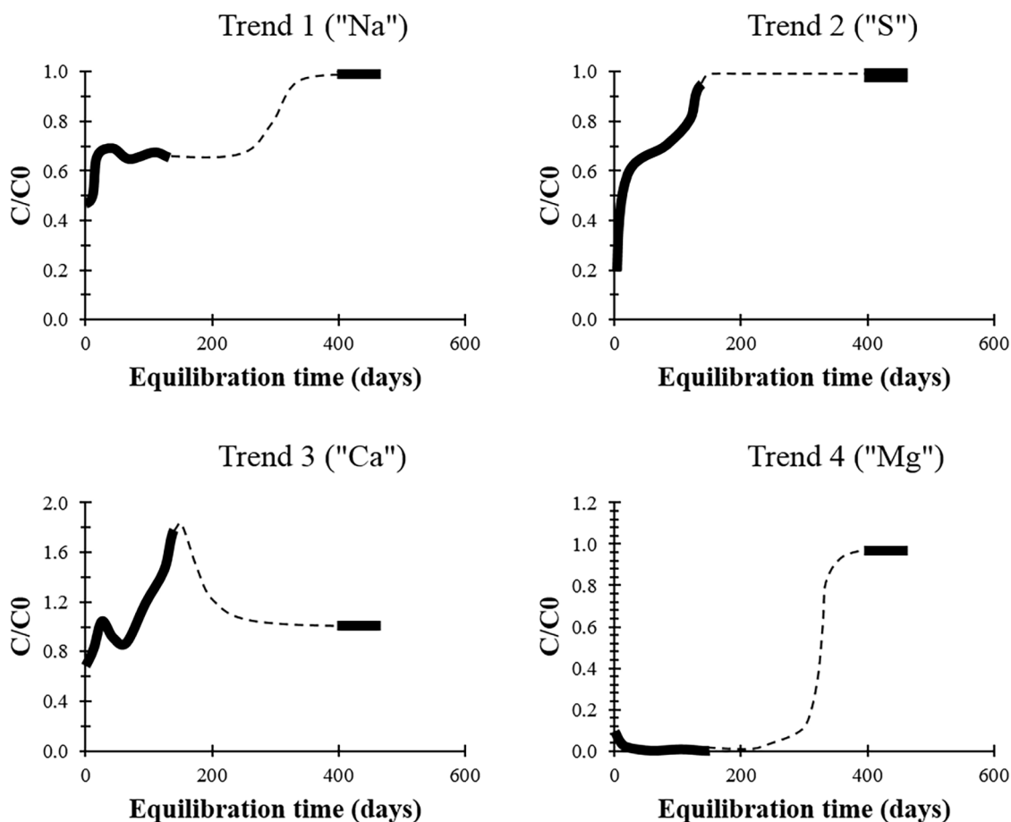
Fig. 8. Trends in major elements and Cr(VI) concentrations in leachate during the pore solution equilibration experiment. Absolute concentrations C are compared to reference concentration C_0 found by initially leaching a fresh sample of COPR using the fast percolation method (see methods and materials). No measurements were made between 140 and 400 days. The lack of data between 140 and 400 days is related to our initially wrong appreciation of kinetic reactions. Indeed, we initially thought that steady state between solid and pore water had been reached after 140 days, because of the observed relative stability of major elemental concentrations (except for calcium and sulfur). Thus after 140 days, we stopped doing measurements. Just out of curiosity, a new measurement was done after 400 days, which revealed that all concentrations had evolved, i.e. , that they had levelled off close to their initial values. It can be concluded that 400 days is about the time needed to reach true steady state conditions in the material. The dashed line is drawn by hand and represents a probable course of the curve. Trend 1 is representative of elements Na, K and Cr(VI). Trend 2 is representative of element S, trend 3 of Ca and trend 4 of Mg. The schematic representations are based on chemical data in Figure S7 (Supplementary Material S7) .
