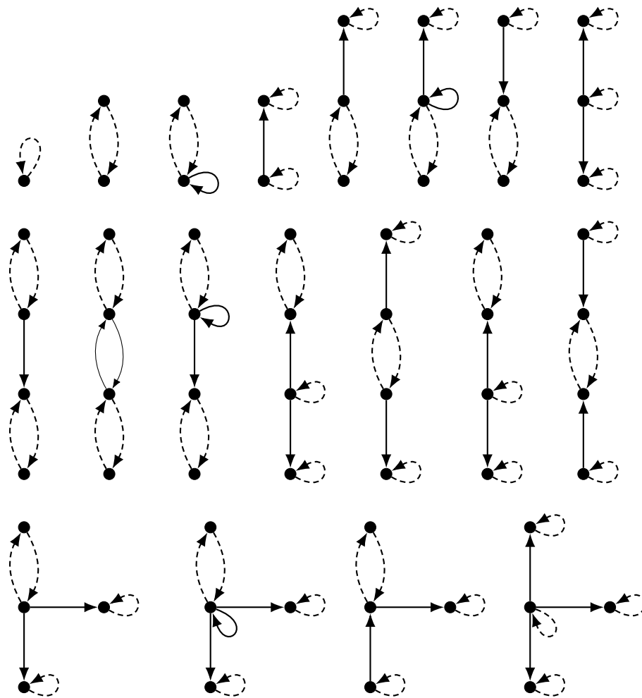
Figure 4: All extremal di-trees with order at most 4. Forcing arcs are dashed.
