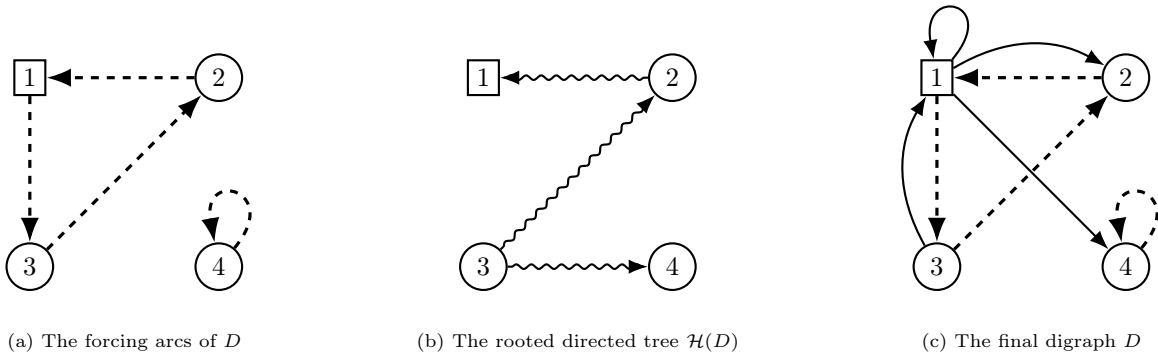
Figure 2: An example of the construction from Theorem 18. The square vertex is the only one in V_d ; the circled vertices are those in V_f ; the dashed arcs are the forcing arcs; the wiggled arcs are those of \mathcal{H}(D) .
