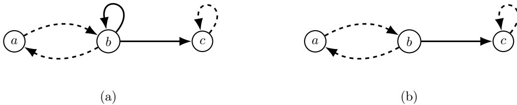
Figure 3: Two extremal di-trees of order 3. Forcing arcs are dashed.
