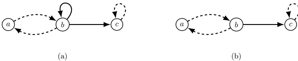
Figure 3: Two extremal di-trees of order 3. Forcing arcs are dashed.
