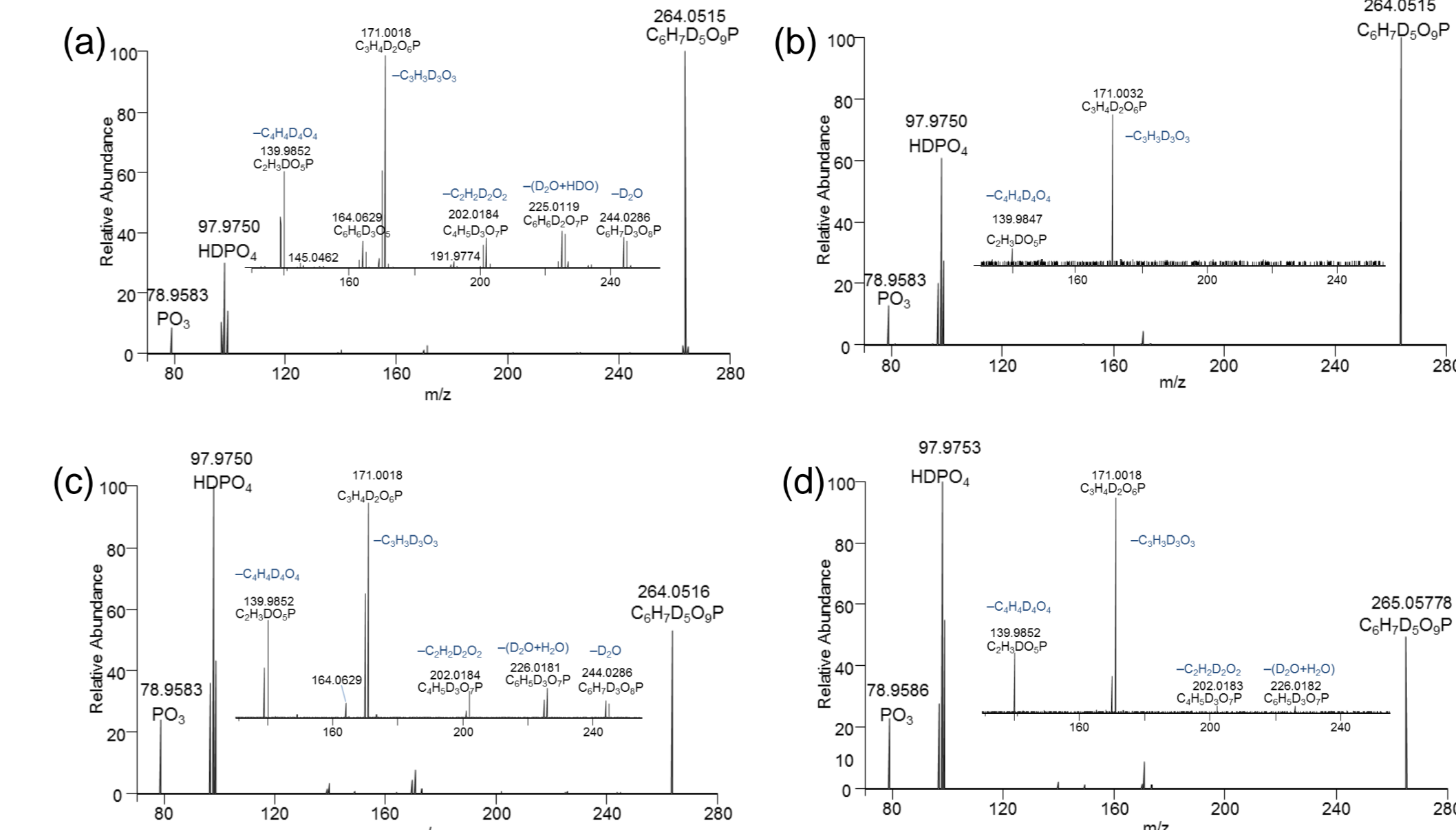
Figure 2. Product ion spectrum (NCE=15% in resonant excitation during 10 ms, CID mode with LMCO at m/z 115) of the d11-labelled sodiated complex (m/z 466).
