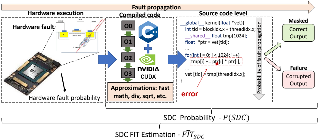
Fig. 1. The CUDA application compiling is performed by NVIDIA CUDA Compiler (NVCC). NVCC translates the high-level C++ code to Shader Assembly (SASS) code to run in a GPU device. In the compilation phases, NVCC also applies a range of optimizations that can be disabled or enabled by the user. Two primary error analyses are considered to evaluate the error propagation: SDC Probability and SDC FIT Estimation. While SDC Probability considers only the software level SASS fault injection and kernel profiling, the SDC FIT Estimation also considers the probability of the fault to be generated in the hardware (instruction FIT rate).
