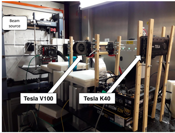
Fig. 1: Experiment setup at ChipIR. More than 1,000 hours of beam experiments are performed for Kepler and Volta GPU architectures. The large beam experiments campaigns allowed obtaining the error rates for 11 HPC codes and 3 CNNs.
