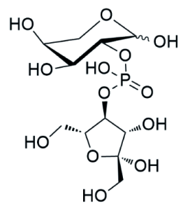
Agrocinopine B
