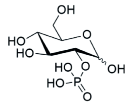
Glucose-2-phosphate
