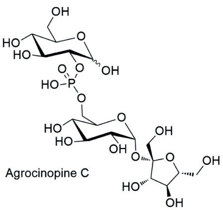
Agrocinopine D
