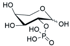
Arabinose-2-phosphate
