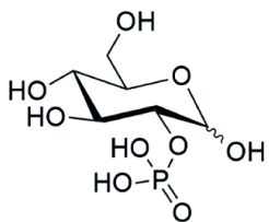
Glucose-2-phosphate
