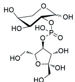
Agrocinopine B
