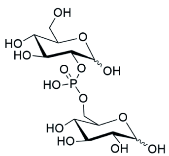
Agrocinopine D
