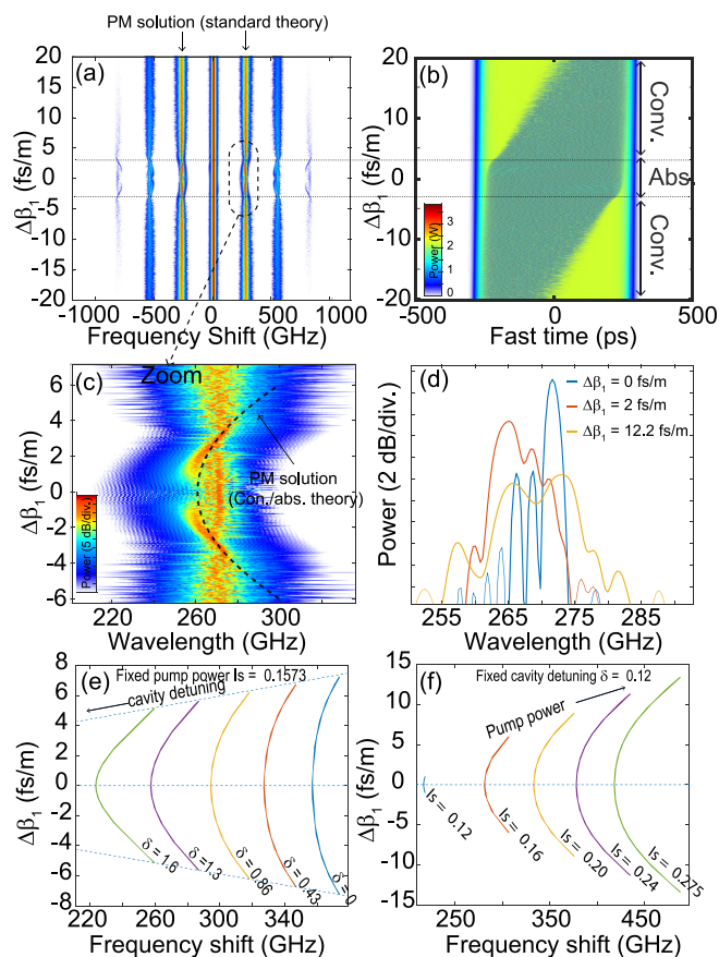
FIG. 1. (a) Evolution of the output spectrum as a function of the group velocity mismatch ( \Delta \beta_1 ) from numerics [LLE integration, Eq. (1)]. (b) Evolution of the output power as a function of the group velocity mismatch. (c) Zoom on a MI sidelobe. The black dashed lines represent theoretical predictions from Eq. (3). (d) Zoom in on the MI sidelobe for different mismatch values (0, 2, 12 fs/m respectively from numerics). (e) and (f) Evolutions of the sidelobe positions and of the absolute regime zone as a function of the cavity detuning and the pump power, respectively, from theory [Eq. (3)]. With \alpha = 0.2327 , \theta = 0.05 , and |E_{\text{in}}|^2 = 2.3 W, extracted from experimental parameters which are all listed in Fig. 2's caption.
