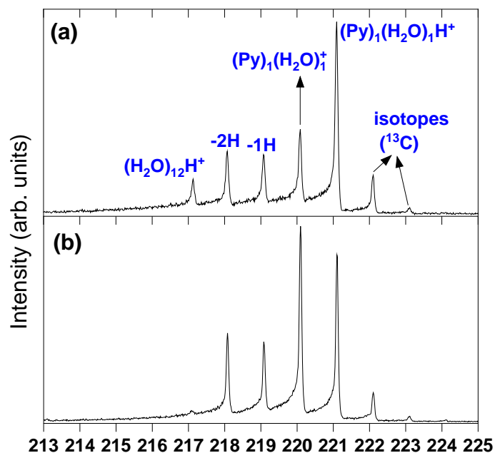
Fig. 4 Zoomed view around the (\text{Py})_1(\text{H}_2\text{O})_1\text{H}^+ species. (a) corresponds to Figure 3(c) and (b) to Figure 3(d)
