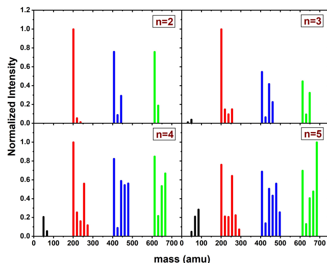
Fig. 10 Mass Distribution of the fragments from CID of (\text{Py})_3(\text{H}_2\text{O})_n\text{H}^+ n=[2-5] on collision with xenon at 7.5 eV COM collision energy. The peaks in the graphs are normalized by the maximum value.
