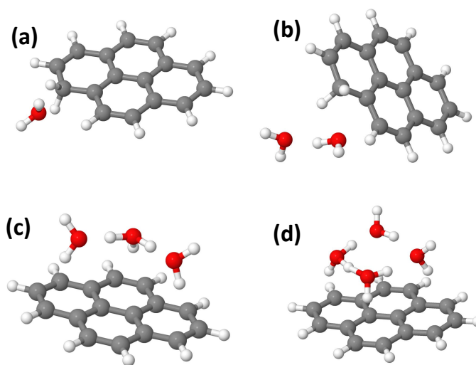
Fig. 12 Lowest energy isomers obtained for (\text{Py})_1(\text{H}_2\text{O})_n\text{H}^+ . (a) n=1 C1, (b) n=2 C1, (c) n=3 C2, (d) n=4 C2. C1 and C2 corresponds to the initial protonation site on the Py molecule. See text for details.
