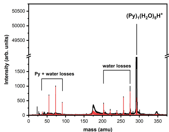
Fig. 5 Fragmentation TOF-MS of (\text{Py})_1(\text{H}_2\text{O})_5\text{H}^+ colliding with argon at E_{\text{COM}}=7.5 eV. The black curve corresponds to the raw data whereas the red curve is obtained after background subtraction. Peaks corresponding to fragmentation are grouped into two channels. Note the break on the vertical scale.
