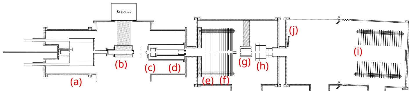
Fig. 1 Schematics of the experimental setup : (a) Cluster gas aggregation source (b) Thermalization chamber (c) First Wiley-McLaren acceleration stage (d) Mass filter (e) Energy focusing (f) Deceleration region (g) Collision cell (h) Second Wiley-McLaren acceleration stage (i) Reflectron (j) Microchannel plate detector.
