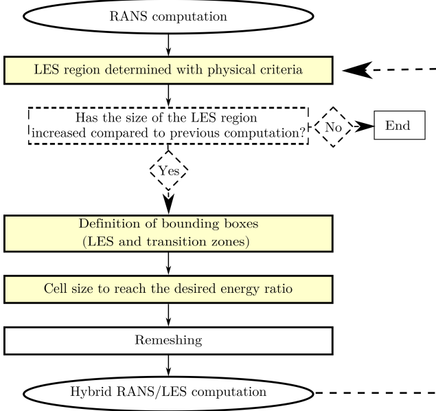
Figure 2: Algorithm used for the self-adaptive approach.
