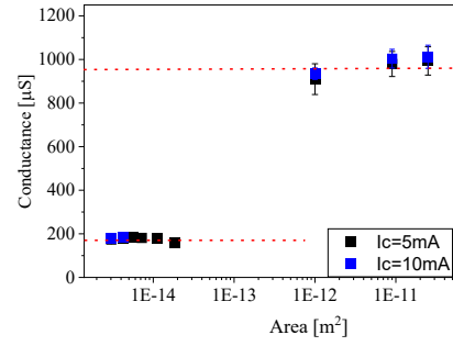
Fig. 6. Conductance as a function of the area during operation of the ReRAM device in the LRS.
