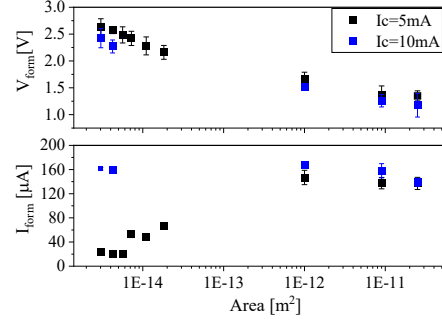
Fig. 4. Area scaling trends for (a) forming voltage ( V_{form} ) and (b) forming current ( I_{form} ), comparing the effect of I_c .
