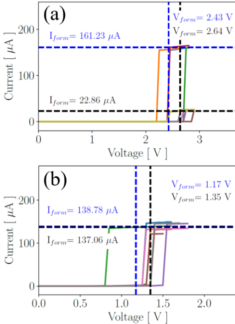
Fig. 3. IV curves during electroforming of two samples (a) 55 \times 55 \text{ nm}^2 and (b) 5 \times 5 \mu\text{m}^2 . The results for I_c = 5 \text{ mA} are in black, while for I_c = 10 \text{ mA} , the results are in blue. One can see that the compliance current significantly affects the response of the nanometer size samples.
