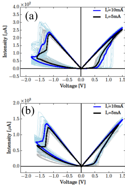
Fig. 5. I-V characteristic for a RRAM device of (a) 55 \times 55 \text{ nm}^2 and (b) 5 \times 5 \mu\text{m}^2 during 50 cycles. The curves show the typical bipolar resistive switching behavior. We cannot identify considerable differences in the transition points, set and reset voltages, and in the LRS region.
