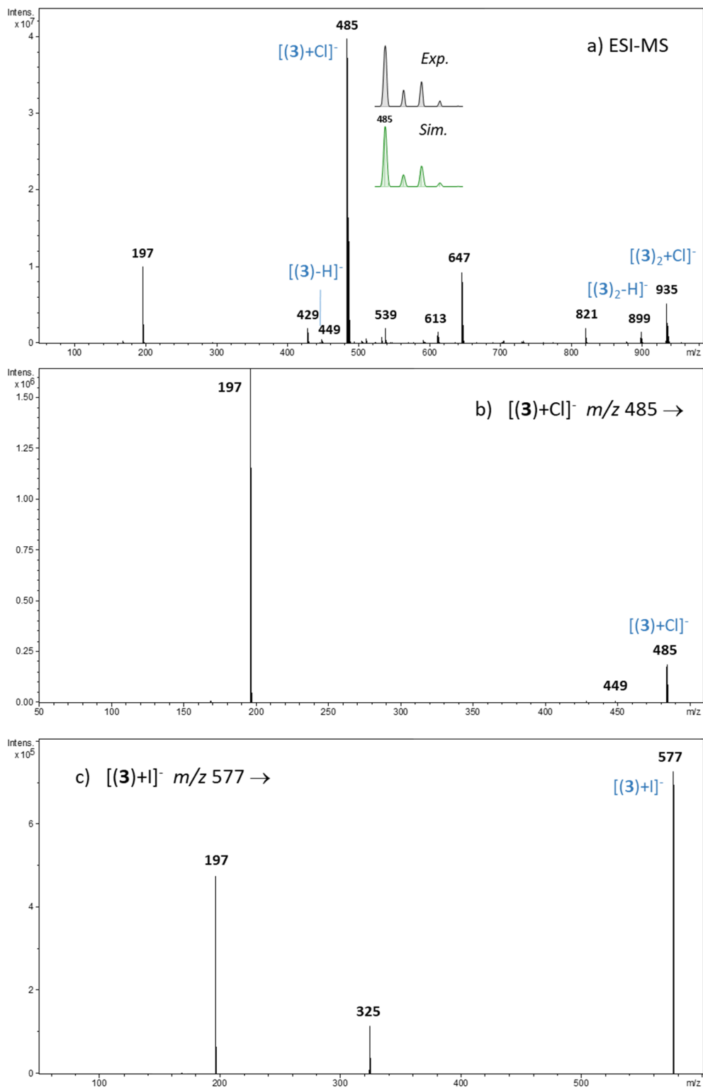
Figure 10 (a) Negative-ion electrospray mass spectrum of an equimolar mixture of 3 /NBu 4 Cl (10 -5 M) in a 90/10 ACN/water solution, MS/MS spectrum of the (b) [(3) + Cl] - ion (m/z 485) and (c) [(3) + I] - ion (m/z 577).
