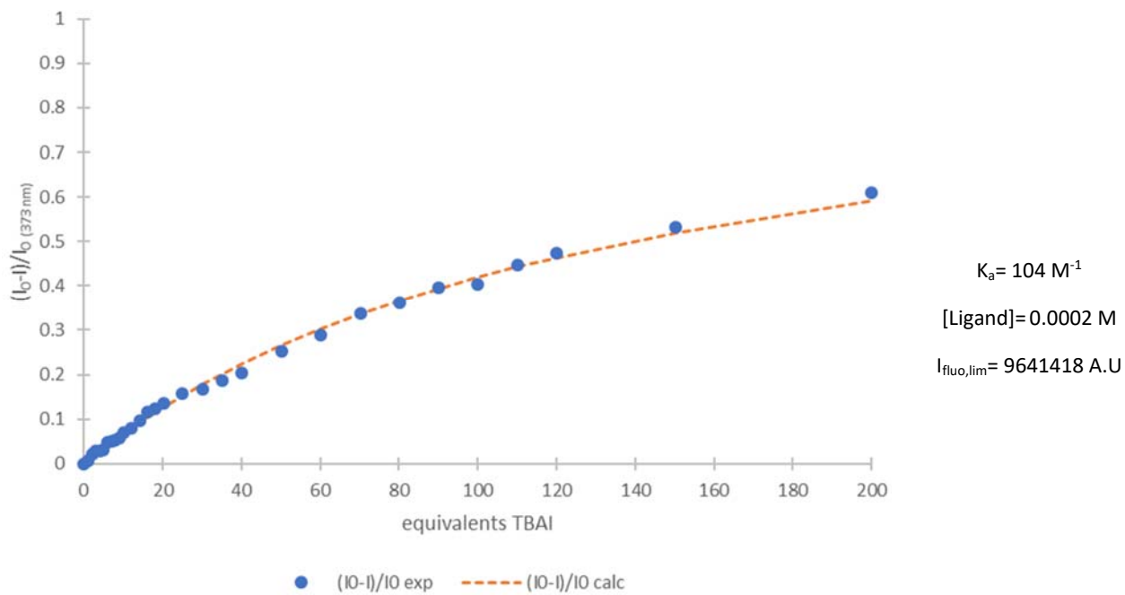
Figure S42 Mathematical fit of fluorescence of 3 with TBAI (from 0 to 200 equivalents) in ACN, ( [3] = 2 \cdot 10^{-4} \text{ M} , \lambda_{\text{exc}} = 325 \text{ nm} ).
