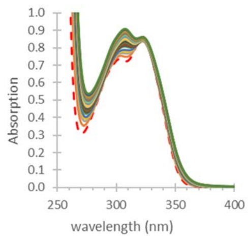
Figure S25 UV-visible titration of 2 with \text{TBACl} (from 0 to 70 equivalents) in ACN, ( [\mathbf{2}] = 2 \cdot 10^{-4} \text{M} )
