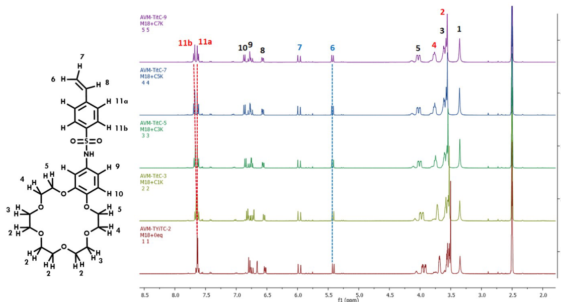
S3: ^1\text{H} -RMN Spectrum (DMSO, 400 MHz) obtained for the titration of the monomer (2) under variable concentrations (from 0 to 2 molar equivalents) of potassium perchlorate.
