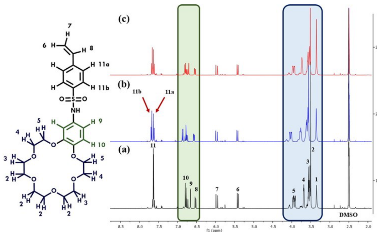
Figure 1. ^1\text{H} -RMN Spectra (DMSO- d_6 , 400 MHz) obtained for monomer (2) in the absence (a) and in the presence of 2 molar equivalents of (b) potassium perchlorate and (c) sodium perchlorate.
