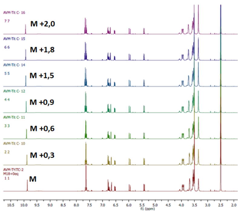
S4: 1 H-RMN Spectrum (DMSO, 400 MHz) obtained for the titration of the monomer (2) under variable concentrations (from 0 to 2 molar equivalents) of sodium perchlorate.
