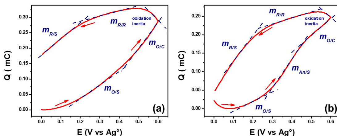
S9: Charge-potential plots of a drop-casted film in a 0.1 M TMAC aqueous solution obtained from the integration of the (a) 1st and (b) 10th potentiodynamic scan.
