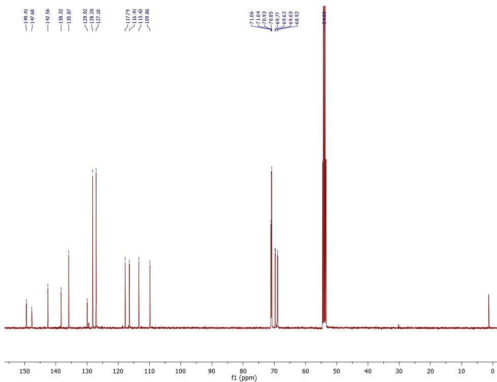
S2 ^{13}\text{C} -NMR ( \text{CD}_2\text{Cl}_2 , 150 MHz) of 4-styrenesulfonyl(phenyl-18-crown-6) imide (2)
