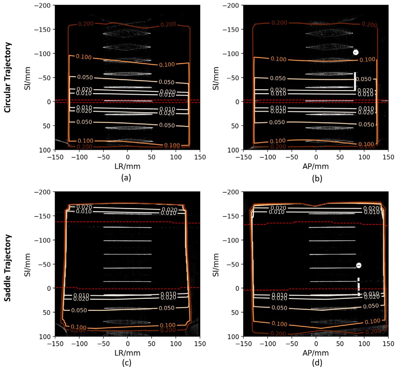
FIGURE 4 Disk phantom with \tan(\psi) plot. (a,b) Coronal and sagittal planes of circular trajectory scan. (c,d) Coronal and sagittal planes of saddle trajectory scan. Solid lines are isolines of \tan(\psi) . Red dashed lines are the edges of the convex hull region. (window level: 0.0082, window width: 0.0136).
