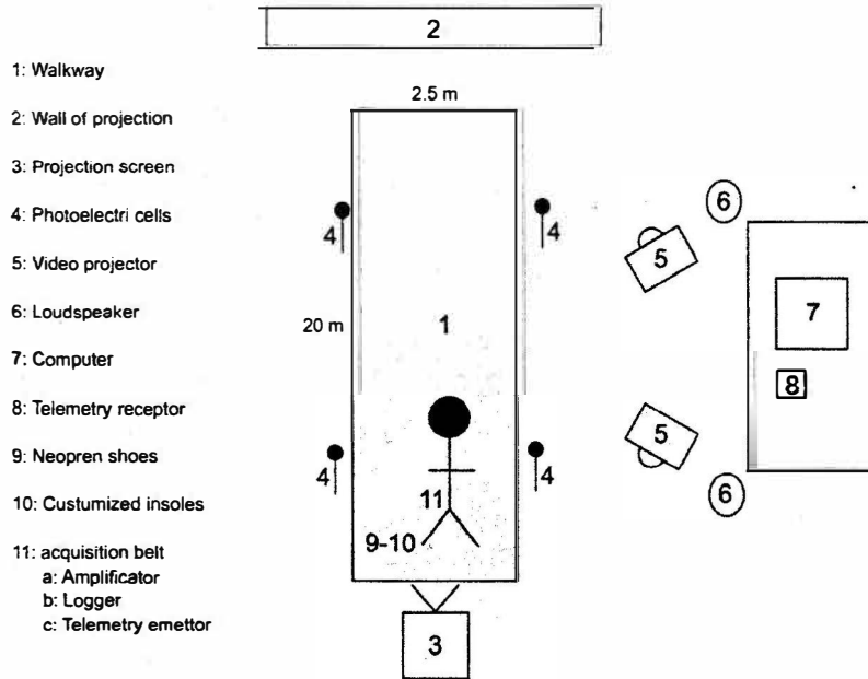
Fig. 3. Instrumentation for the walking test
