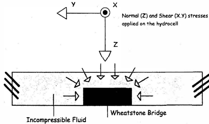
Fig 1. Hydrocell from paromed
