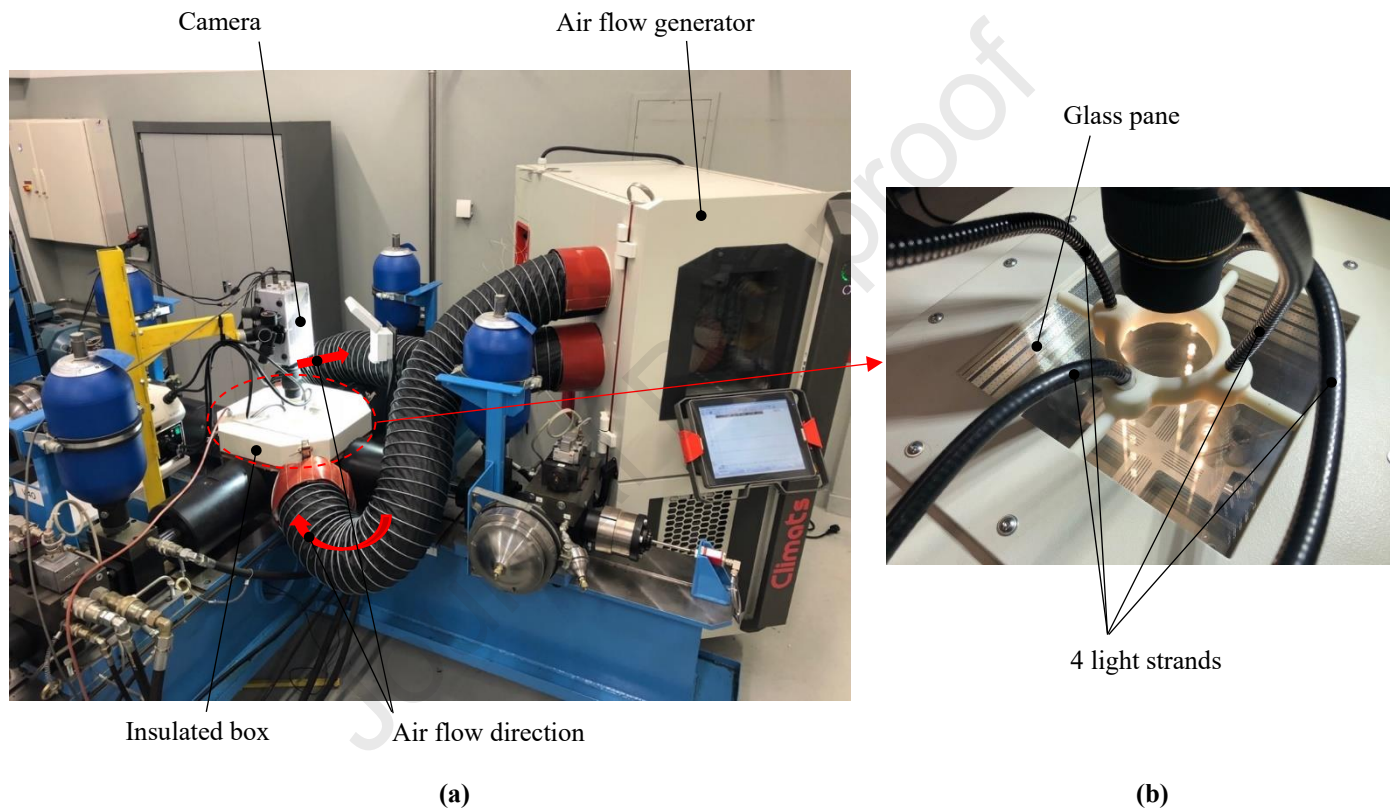
Fig. 2 Biaxial tensile machine equipped with heating device.
