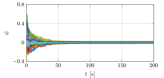
Fig. 2: Estimation errors of the interconnection weights.
