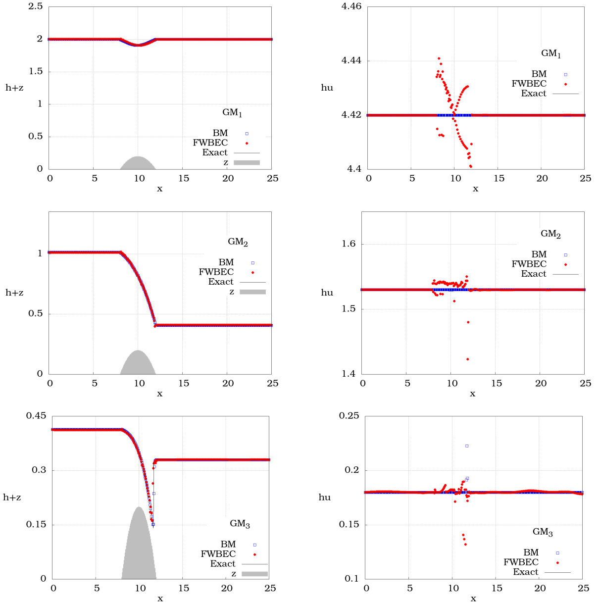
Figure 7: Numerical results for the Goutal and Maurel's problems (90) on a mesh composed of 400 cells. The legend is FWBEC: fully well-balanced entropy satisfying solver given by Theorem 6.1, BM: scheme derived in [14] associated to the Rusanov numerical flux [44].
