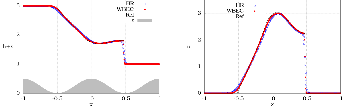
Figure 5: Numerical results at time 0.1 for the break dam problem (91) on a mesh made of 400 cells with the legend WBEC: Theorem's 5.1 solvers, HR: hydro-static reconstruction [3] with the Rusanov numerical flux [44].
