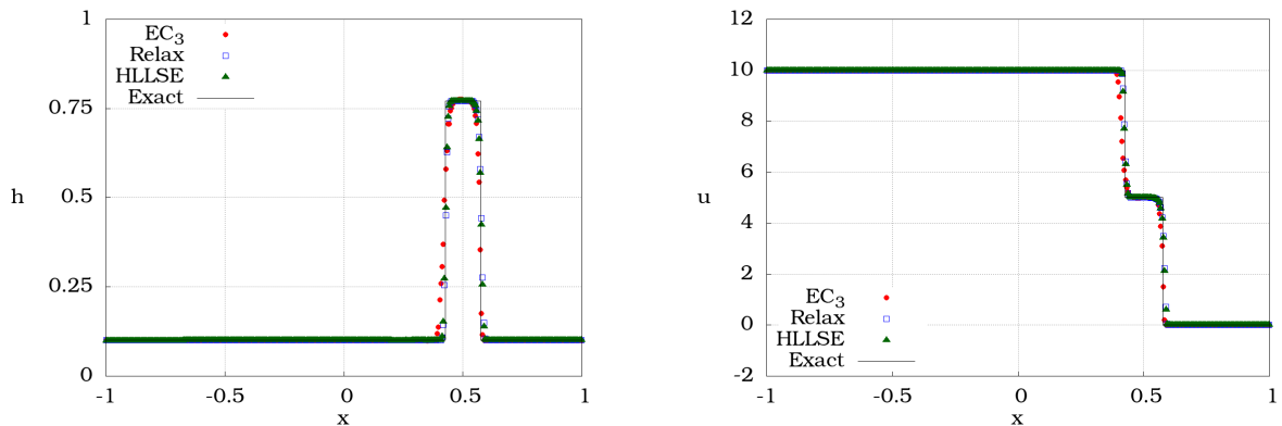
Figure 2: Numerical results at time 0.1 for the initial condition (88), with the legend EC_3 : Lemma’s 4.2 solvers, Relax: Suliciu relaxation scheme and HLLSE: solver [29, Section b.ii].
