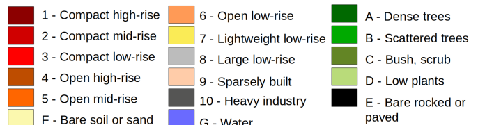
Fig. 1. Local Climate Zones classes
