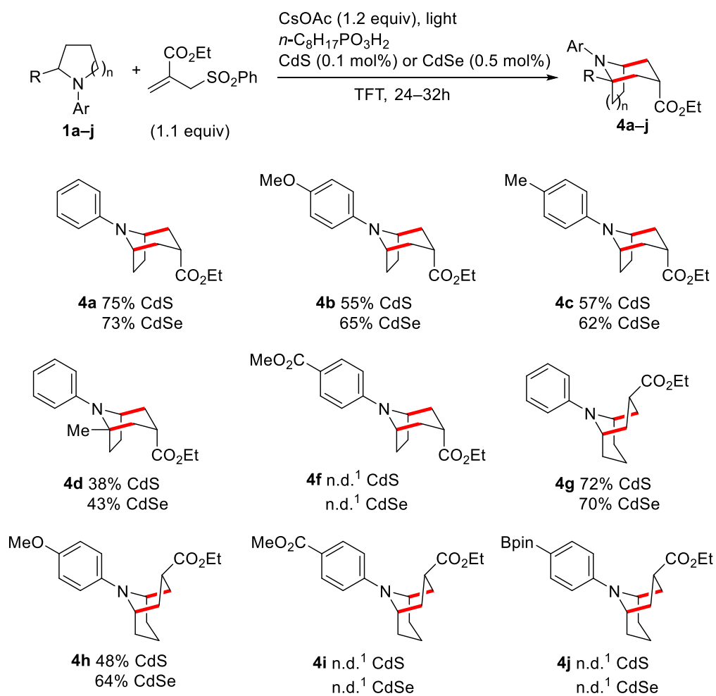
Scheme 2. Reaction scope with N -arylamines (1 \mu mol scale, yields determined by UHPLC-MS). 1 n.d. = not detected.
