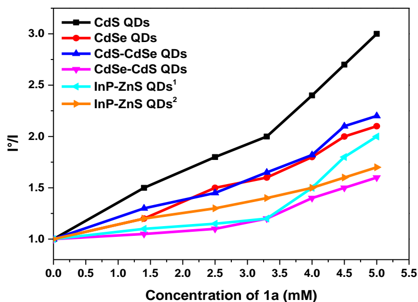
Figure 2. Photoluminescence quenching of the QDs by 1a . Stern-Volmer plots computed from the photoluminescence plot (see SI 2 for details) of the QDs in presence of 1a (up to 5 mM) in TFT. 1 Oleylamine capped InP-ZnS QDs. 2 Commercial oleate capped InP-ZnS QDs.
