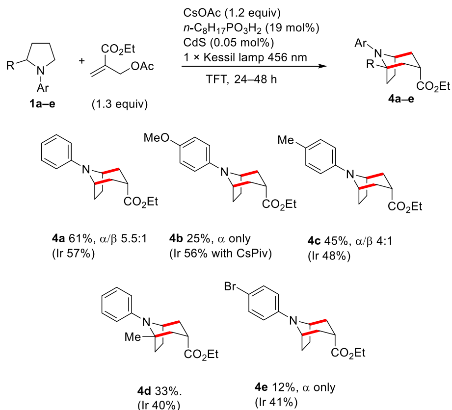
Scheme 3. Substrate scope with N -arylpyrrolidines (50 \mu mol) using CdS QDs. Yields given for the iridium-catalyzed reactions are taken from previous work [40]
