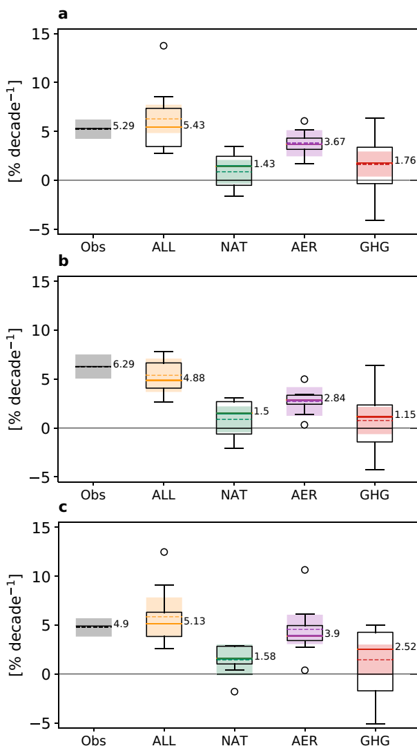
FIG. 10. The 1980–2014 trends of the daily rainfall 10-yr return level ( \% \text{ decade}^{-1} ) derived from the RNSGEV model fitted on two-member samples of annual maxima daily rainfall for each model over (a) the whole Sahel, (b) western Sahel, and (c) eastern Sahel. Boxplot diagrams show the intermodel spread for ALL, NAT-, AER-, and GHG-only simulations: box is the first (Q1)–third (Q3) interquartile range (IQR), whiskers extend from Q1 - 1.5 \times \text{IQR} to Q3 + 1.5 \times \text{IQR} . The median trend across models is indicated with the plain line and number aside. Shading depicts the uncertainty due to RNSGEV model inference for observations (gray) and models (color). Dashed lines indicate the median across 200 bootstrapped trend values.
