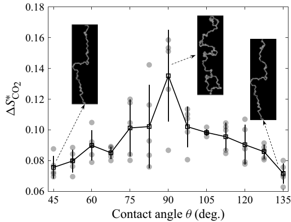
Figure 8. Terminal saturation hysteresis \Delta S^*_{CO_2} for different contact angles. Error bars represent standard deviation. Insets show examples of the active area during cyclic injections for contact angles \theta = \{45^\circ, 90^\circ, 135^\circ\} .
