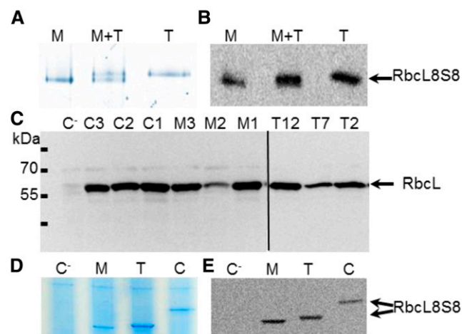
Figure 4. Electrophoretic analysis of leaf, trichome, and C. reinhardtii Rubisco. A, Native gel electrophoresis of soluble proteins from leaf tissues cleared of trichomes (M; 3 \mu g), from isolated trichomes (T; 30 \mu g). A mix of 1.5 \mu g of soluble proteins from leaf tissues cleared of trichomes and 15 \mu g of soluble proteins from isolated trichomes (M+T) was also analyzed in order to confirm that trichome and mesophyll Rubisco complexes are electrophoretically distinct. The gel was stained with colloidal blue. B, An electrophoresis performed as in A was followed by western blotting using an anti-RbcL antibody. C, Western blotting analysis of RbcL in the C. reinhardtii lines. Soluble proteins (40 \mu g) from pSS1-CrRbcS1 (C1, C2, and C3), pSS1-NtRbcS-M (M1, M2, and M3), and pSS1-NtRbcS-T (T2, T7, and T12) transformants were analyzed by SDS-PAGE and western blotting using an anti-RbcL antibody. The recipient strain (C - ) lacking RbcS genes was used as a negative control. D and E, Native gel electrophoresis of soluble proteins (40 \mu g protein) from C. reinhardtii transformants. Soluble extracts of the recipient strain lacking RbcS genes (C - ), strains expressing pSS1-NtRbcS-M (M), pSS1-NtRbcS-T (T), or pSS1-CrRbcS1 (C) were electrophoresed on a native gel and either stained with Coomassie Blue (D) or subjected to western blotting using an anti-RbcL antibody (E).
