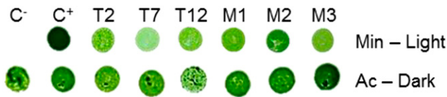
Figure 5. Tobacco RbcS-T and RbcS-M allow light-driven growth of C. reinhardtii . The recipient strain ( C^- ) lacking the RbcS genes and the strains transformed with pSS1-CrRbcS1 ( C^+ ), pSS1-NtRbcS-T (T), or pSS1-NtRbcS-M (M) were spotted on either a minimal medium (Min) under light ( 75 \mu\text{E m}^{-2} \text{s}^{-1} ), or on an acetate medium (Ac) under dark conditions and grown for 11 d.
