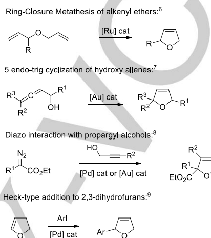
Scheme 1. Usual approaches towards 2,5-dihydrofurans
