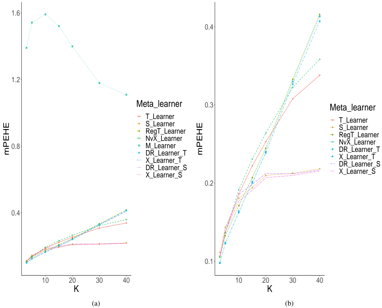
Figure 1. Variation of meta-learners' performances as functions of the number of possible treatment values K for the hazard rate function in an observational design setting. (a): All meta-learners; (b): Without the M-learner
