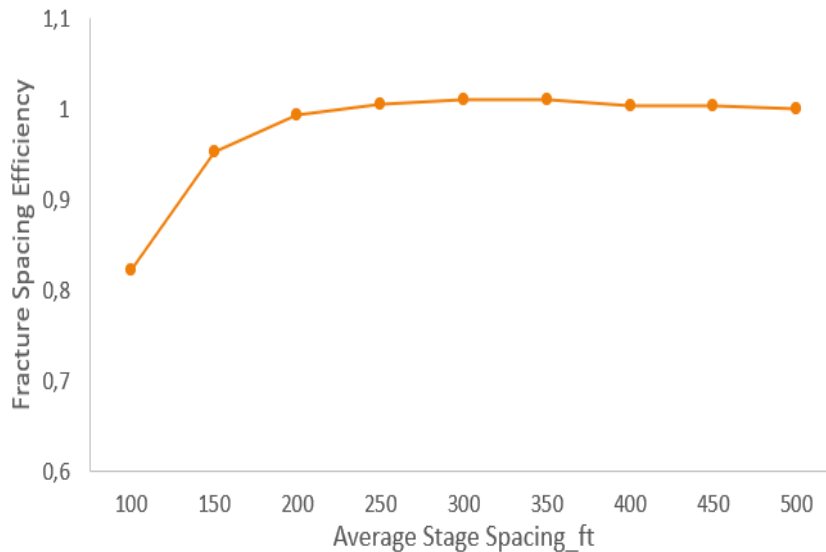
Figure 4. Cross plot between fracture spacing efficiency and average stage spacing.
