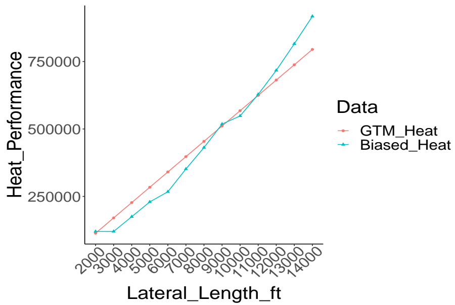
Figure 5. An illustration of selection bias on the heat performance. Red line: The heat extraction performance on the main dataset (i.e. Ground Truth Model). Blue line: The heat performance on the biased dataset (i.e. observed response).
