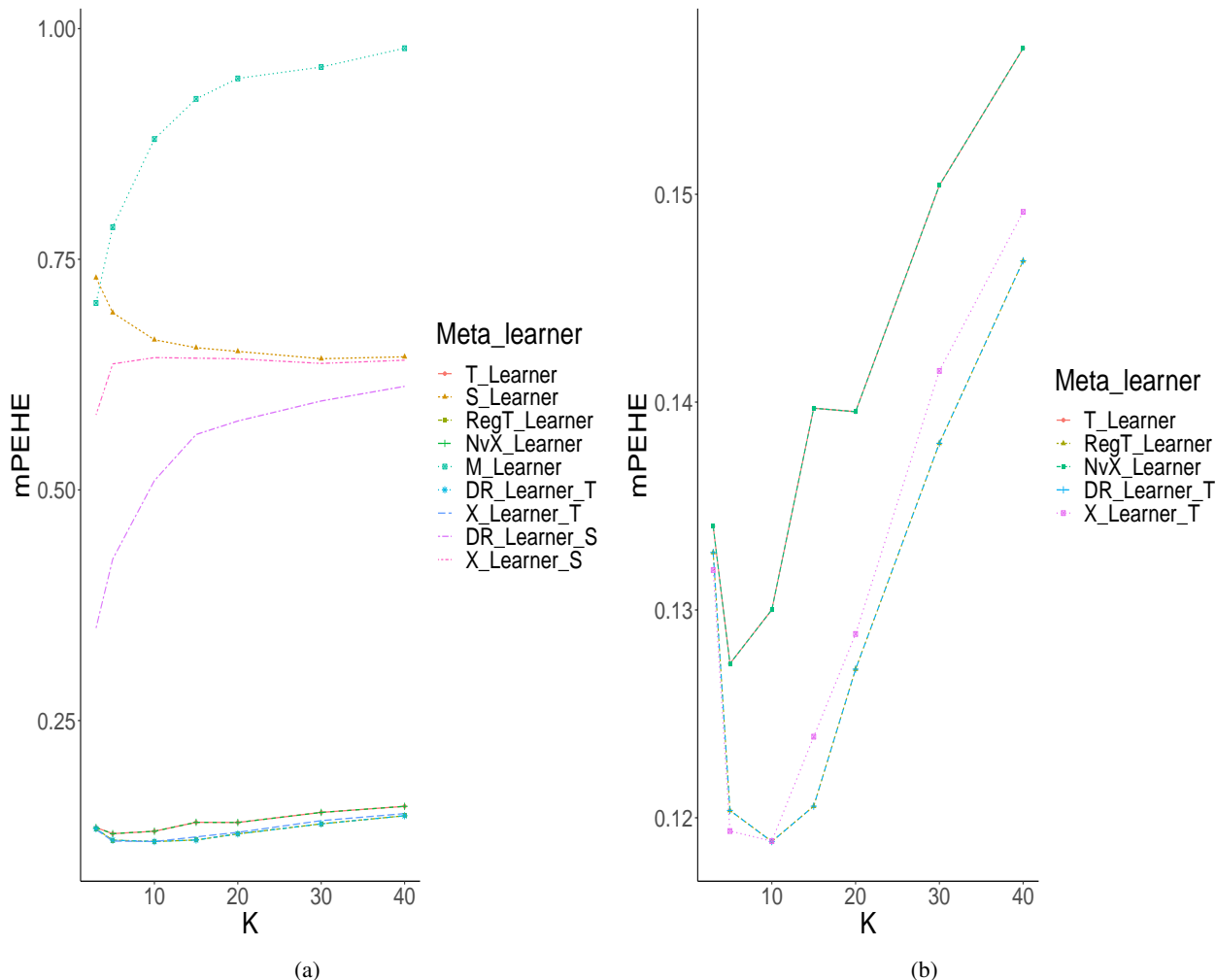
Figure 2. Variation of meta-learner’s performances when the number of possible treatment values K for the hazard rate function in observational design setting with a linear model. (a): All meta-learners; (b): Focus on the T-learning methods.
