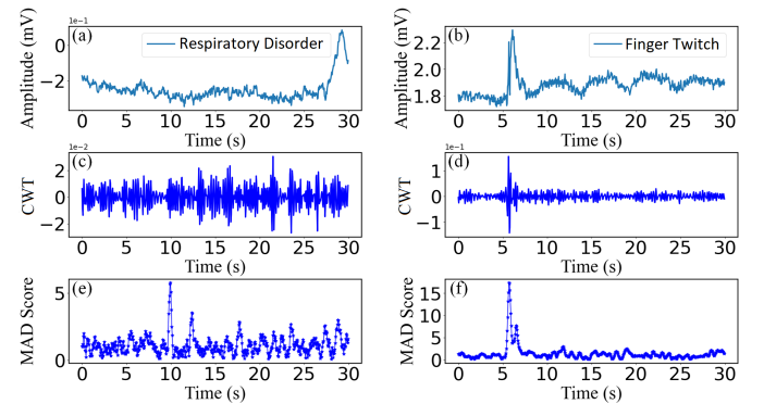
Fig. 14: Signal waveforms before and after CWT and MAD processes. Original signal of (a) respiratory disorder and (b) finger twitch movement. CWT waveforms of (c) respiratory disorder and (d) finger twitch movement. MAD results of (e) respiratory disorder and (f) finger twitch movement.
