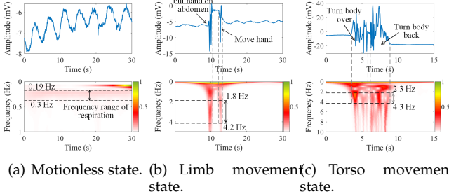
Fig. 13: Signal waveforms and CWT scalograms under different body states.
