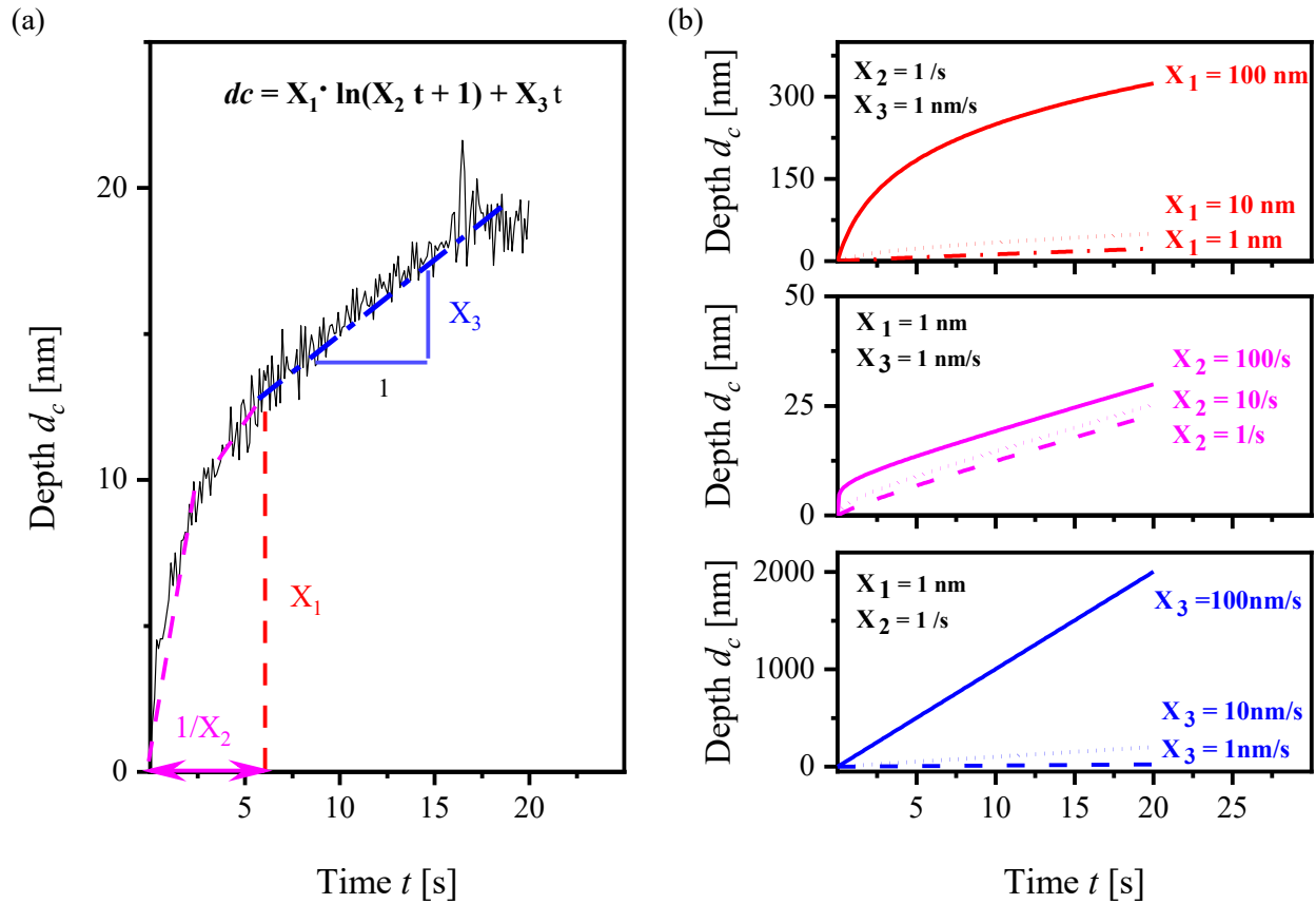
Figure 8. Indentation creep deformation. (a) The time-dependent creep deformation is captured using a three-parameter creep model. (b) Creep deformation was calculated with unitary, tenfold, and hundredfold values of the constants X_1 [nm], X_2 [1/s], and X_3 [nm/s] to illustrate their control of the creep behavior.
