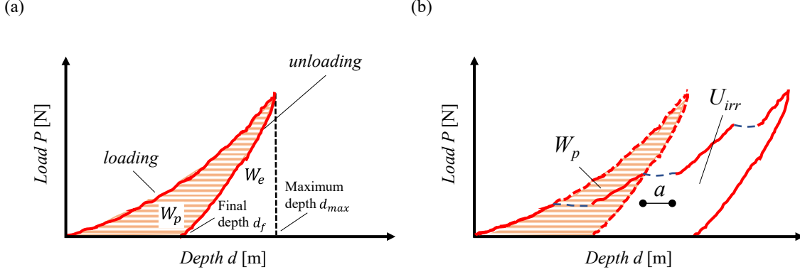
Figure A-1 Indentation energy in a loading-unloading cycle. (a) Total energy distributed in elastic energy W_e during material unloading rebound and plastic energy W_p caused by plastic mechanisms excluding major cracking events. (b) Plastic energy W_p and irrecoverable energy U_{irr} including cracking events of approximate length a .
