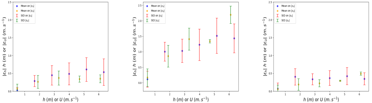
Figure 22: Error metrics in space and time on predicted flow variables in the online phase. Comparison of complexity between (left) Setup 1: EA-POD-NN with N_{rb} = 5 and N_{er} = 10 , (middle) Setup 2: POD-NN with N_{rb} = 10 and (right) Setup 3: POD-NN with N_{rb} = 63 in the non-simultaneous inflows case at maximum flooding time for \mu_{new} = (8.66, 1100, 8.38, 300, 22.2) (red point in Fig. 11). The histogram of the mean and the StD of spatial values of the absolute difference |\varepsilon_h| and |\varepsilon_U| at maximum flooding time. (Left) Setup 1 The difference \varepsilon_h or \varepsilon_U for EA-POD-NN \mathbf{u}_{h,EA-POD-NN}(\mu_{new}) with N_{rb} = 5 and N_{er} = 10 . (Middle) Setup 2 The difference \varepsilon_h or \varepsilon_U for POD-NN \mathbf{u}_{h,POD-NN}(\mu_{new}) with N_{rb} = 10 . (Right) Setup 3 The difference \varepsilon_h or \varepsilon_U for POD-NN \mathbf{u}_{h,POD-NN}(\mu_{new}) with N_{rb} = 63 .
