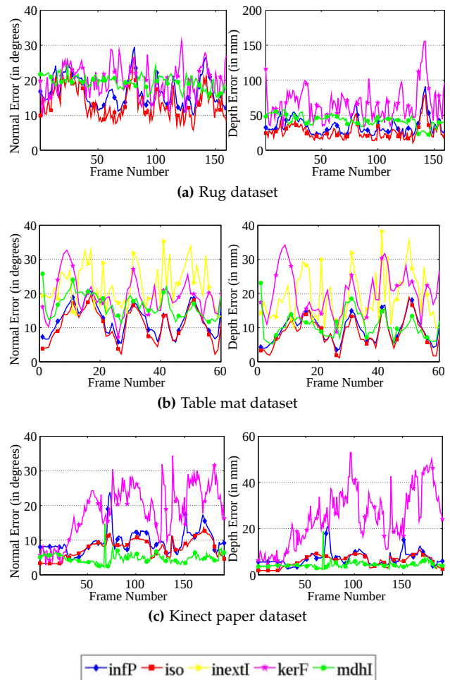
Fig. 7: Experiments on long sequences. The average normal and depth error for each frame is shown. The experiment with inextI is only performed for the table mat dataset. Best viewed in colour.
