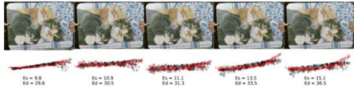
Fig. 9: Experiment with an almost stationary object. The first five images of the table mat sequence are used. The reconstruction of iso is shown in red. The ground truth is indicated with black. E_s represents the mean shape error (in degrees). E_d represents the mean depth error (in mm). The performance of iso is almost the same as infP on these five images.
