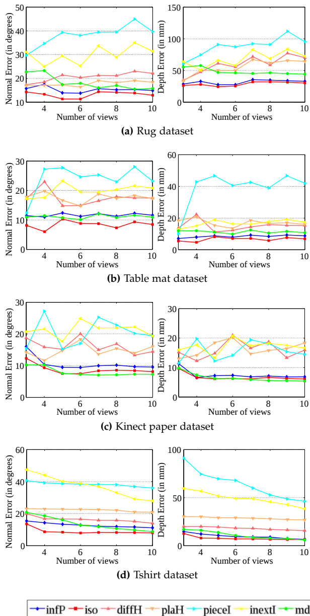
Fig. 5: Experiments on short sequences. The average normal and depth error for each experiment with number of views varying between 3-10 is shown. The views of the rug, table mat and kinect paper datasets are selected by uniform sampling the long sequences. The views of the tshirt dataset are selected by randomly sampling the dataset and the results are averaged over 20 trials. Best viewed in colour.
