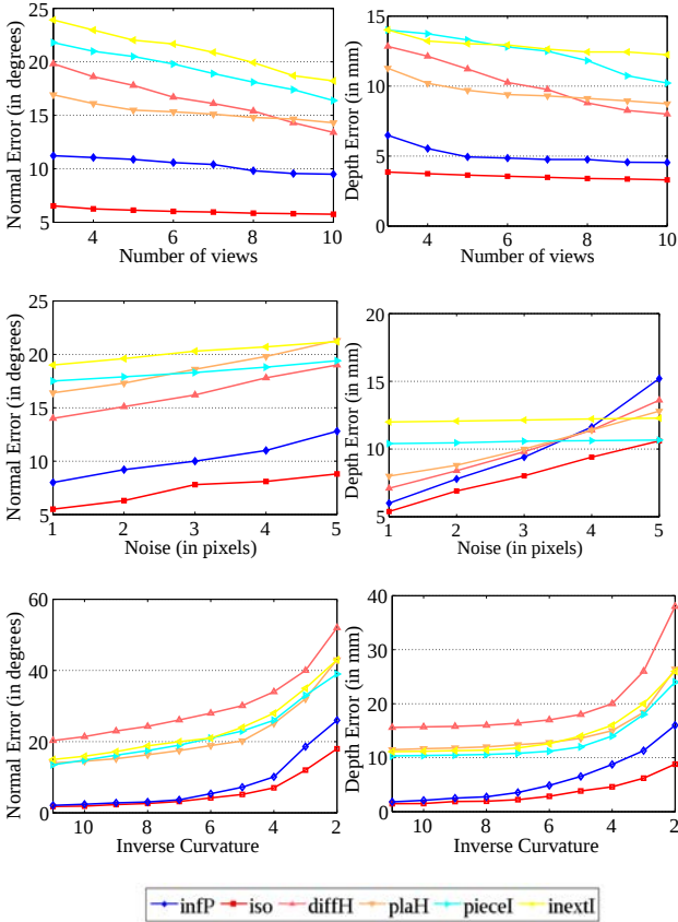
Fig. 4: Synthetic data experiments. Average normal and depth errors with respect to number of views, noise and curvature. Best viewed in colour.
