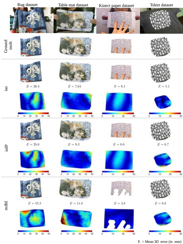
Fig. 6: Reconstruction error maps and renderings for the rug, table mat, kinect paper and tshirt datasets. We remind that mdhI reconstructs only the visible part of the surface. Therefore, the rendering and error map for the kinect paper dataset is broken for this method.
