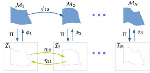
Fig. 1: The proposed model of NRSfM, where each surface \mathcal{M}_i is a Riemannian manifold defined by embedding the corresponding retinal plane \mathcal{I}_i .
