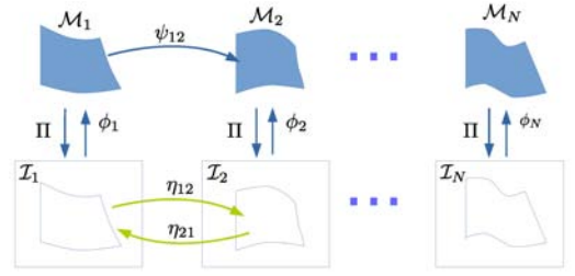
Fig. 1: The proposed model of NRSfM, where each surface \mathcal{M}_i is a Riemannian manifold defined by embedding the corresponding retinal plane \mathcal{I}_i .
