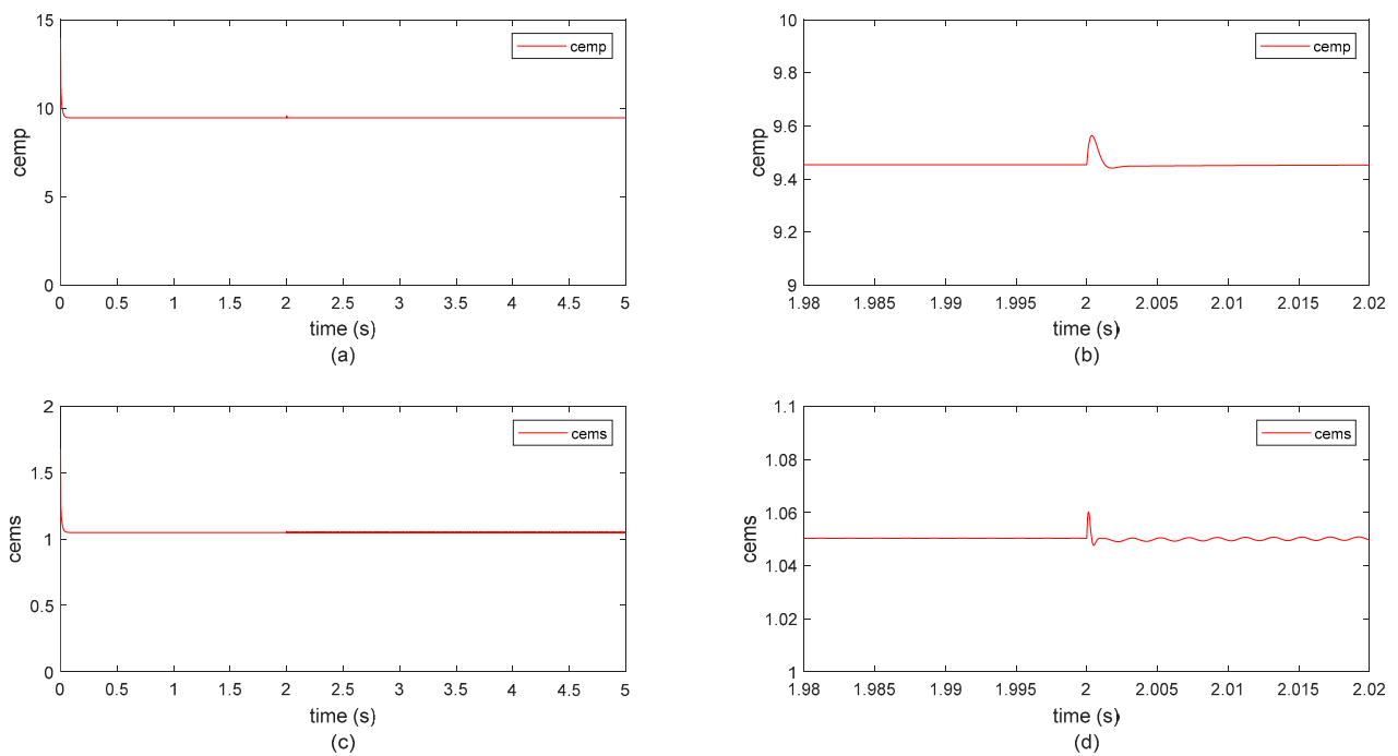
Figure 7. The electromagnetics torques’ components ( c_{emp} (a,b) and c_{ems} (c,d)) in the presence of stator faults with the optimization of PI controller parameters using the GWO algorithm.
