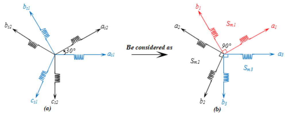
Figure 2. Model of the DSIM: (a) two three-phase windings and (b) multi-biphas grouping.
